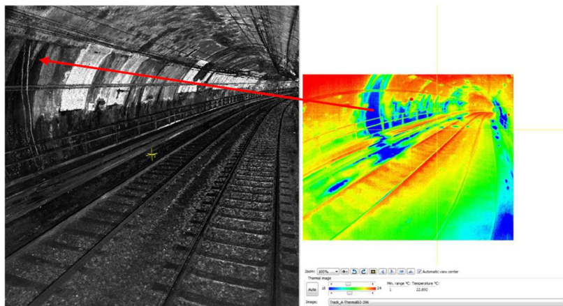
Figure 9: Comparison of a) HD-resolution images and b) thermal images for defect detection.
