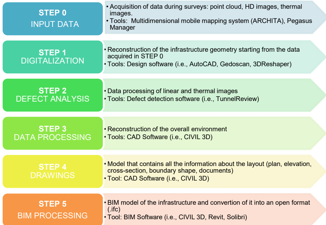
Figure 1: Workflow of SCANToBIM.
