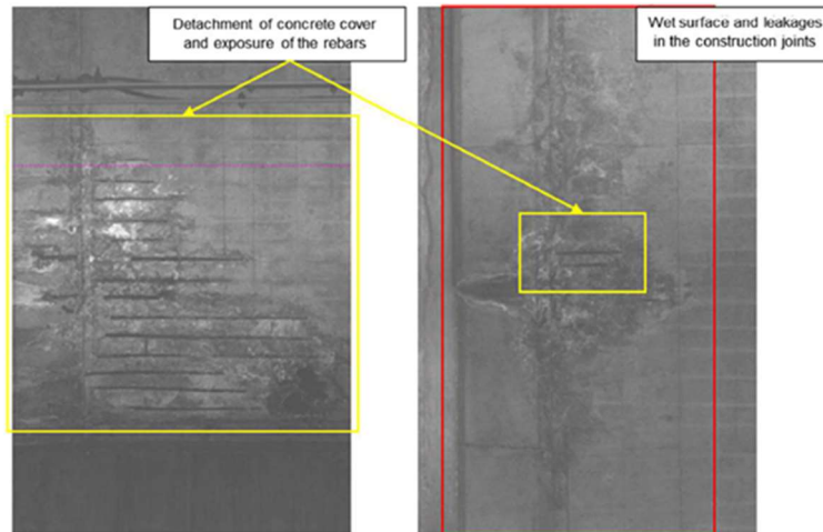
Figure 7: Example of defects: Detachment of concrete cover and exposure of the rebars (yellow) and Wet surface and leakages in the construction joints (red).
