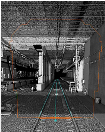
Figure 12: Overlay of the design gauge on a cross-section in 3DReshaper.
