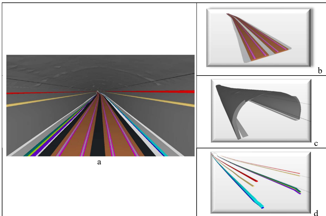
Figure 18: 3D model of a tunnel track on Solibri; a) overall model; b) rails, fasteners, and sleepers; c) civil works; d) lifelines and systems.
