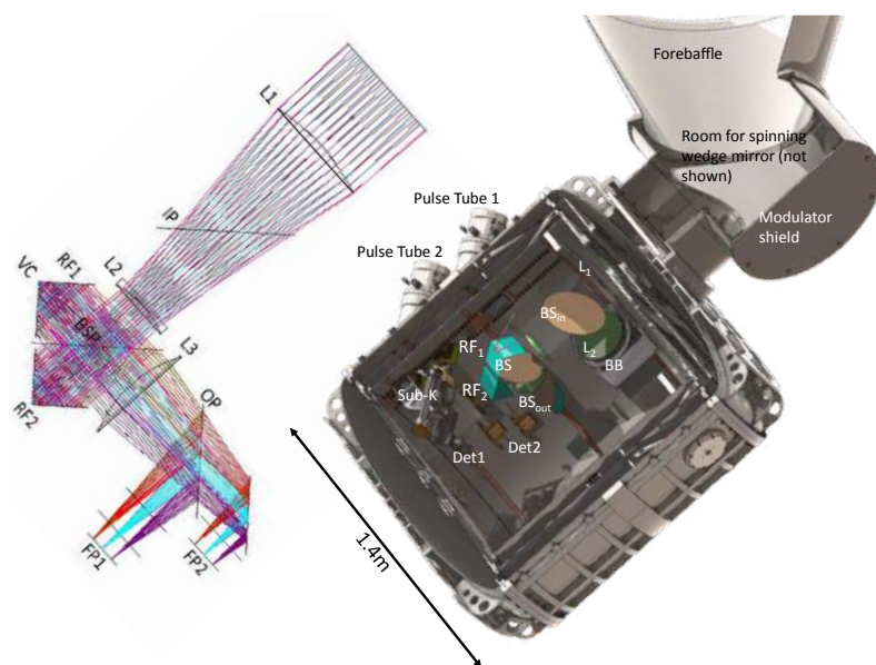
Fig. 5. Left: Ray tracing and optical design of COSMO. L1 is the light collector lens, L2 produces a nearly parallel beam for the FTS, L3 focuses radiation of the focal planes FP1 and FP2. The Differential Fourier Transform Spectrometer is constituted by the input polarizer IP, the beam-splitter polarizer BSP, the roof mirrors RF1 and RF2, the output polarizer OP. The input polarizer transmits radiation from the sky and reflects radiation from the cryogenic reference blackbody. Right: rendering of the accommodation of the COSMO instrument inside its cryogenic system.
