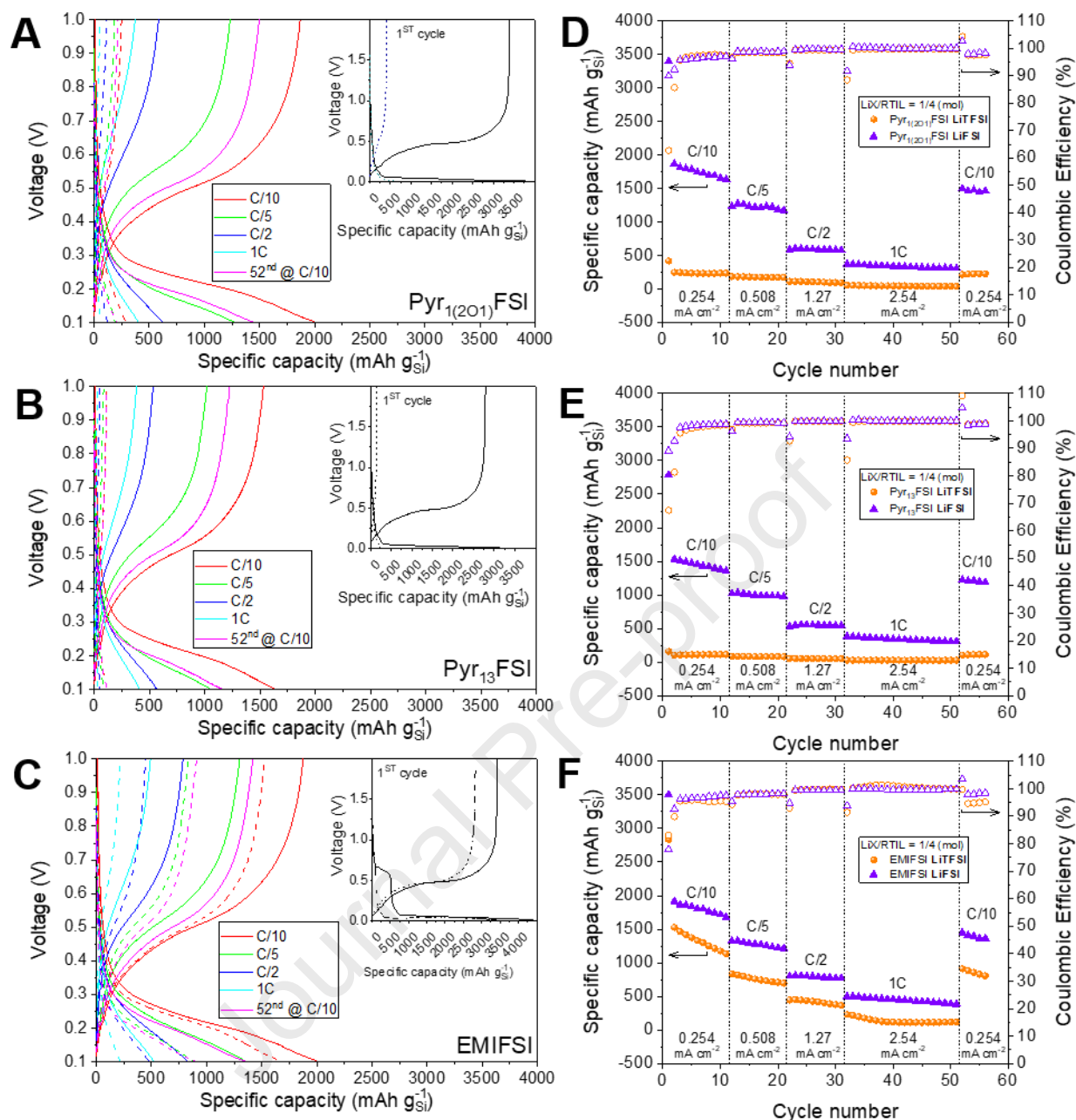
Figure 4 – Voltage vs. gravimetric specific capacity profiles during the CC cycling in the range 0.01–2 V vs. Li + /Li 0 (1 st cycle at C/10 i.e. 250 mA g Si -1 , insets) and 0.1–1 V vs. Li + /Li 0 (following cycles at different C-rates) of Li/electrolyte/SiGPAA half-cells (A-C) and corresponding gravimetric specific de-lithiation capacity and Coulombic efficiency vs. cycle number (D-F). The RTIL-based electrolytes contain either LiTFSI (dashed lines in A-C, orange in D-F) or LiFSI (solid lines in A-C, violet in D-F) dissolved in (A,D) Pyr 1(201) FSI, (B,E) Pyr 13 FSI, or (C,F) EMIFSI. Open symbols = Coulombic efficiency, solid symbols = de-lithiation specific capacity. The gravimetric specific capacity is referred to the active Si content only. The SiGPAA mass loading is 2.54 mg cm -2 ( \approx 1.0 mg Si cm -2 ; maximum practical capacity \approx 2.5 mAh cm -2 in the range 0.1–1 V vs. Li + /Li 0 ).
