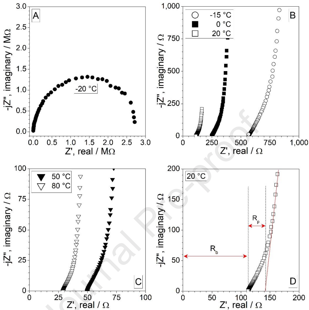
Figure 1 – Representative Nyquist diagrams ( Z' vs. -jZ'' ) of the impedance responses obtained for the LiFSI-EMIFSI electrolyte in a conductivity cell with porous Pt electrodes at: A) -20\text{ }^\circ\text{C} below the melting point; B) different temperatures in the range between the melting point and 20\text{ }^\circ\text{C} , as noted in the legend; C) different high temperatures as noted in the legend, D) 20\text{ }^\circ\text{C} , including the fitting lines and the attribution of the spectral features to the bulk resistance ( R_b ) and resistance due the electrode surface roughness behaving as a porosity ( R_p ).
