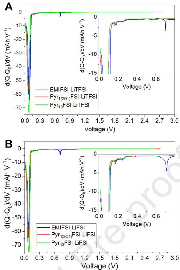
Figure 3 – Derivative dQ/dV curves corresponding to the first CC lithiation of SiGPAA (mass loading 1.03 \text{ mg cm}^{-2} , i.e. 0.41 \text{ mg}_{\text{Si}} \text{ cm}^{-2} ) in Li/electrolyte/SiGPAA half-cells containing (a) LiTFSI or (b) LiFSI at low current density ( 0.047 \text{ mA cm}^{-2} , i.e. 115 \text{ mA g}^{-1}_{\text{Si}} ) with a cut-off voltage of 0.01 \text{ V vs. Li}^+/\text{Li}^0 . The insets show a magnification in the range 0\text{-}0.8 \text{ V vs. Li}^+/\text{Li}^0 .
