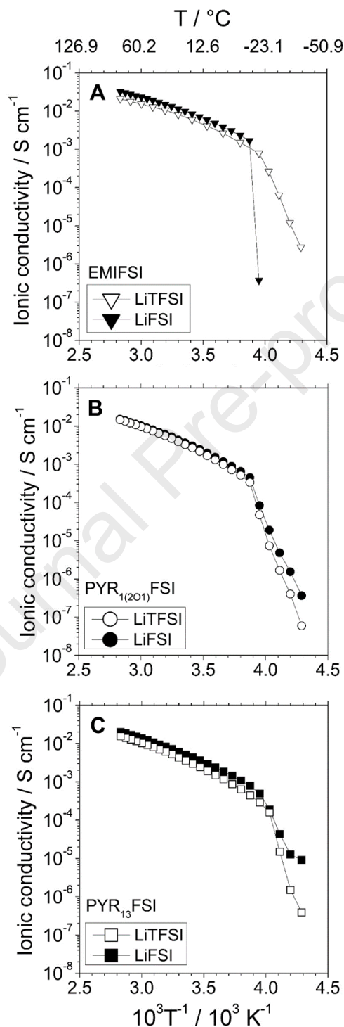
Figure 2 – Arrhenius plot of the ionic conductivity data extracted from the analysis of the electrochemical impedance response of conductivity glass cells with porous Pt electrodes filled with different RTIL-based electrolytes containing LiTFSI or LiFSI as noted in the legend.
