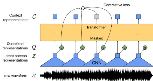
Figure 4: Wav2vec 2.0 pipeline
