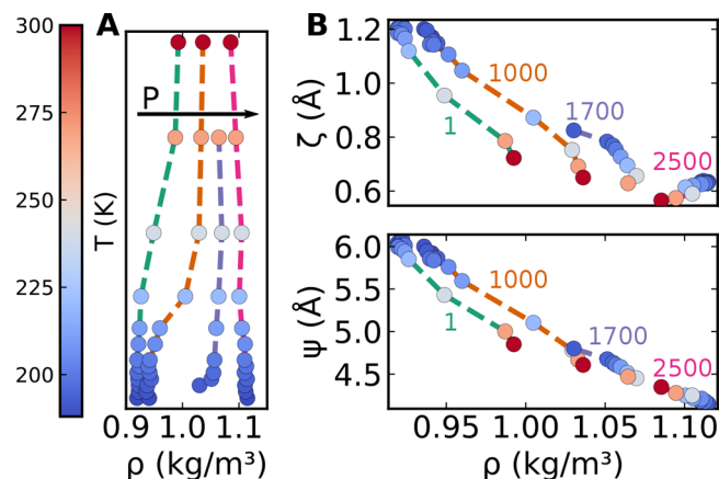
Figure 8. Structural indicators away from the LLCPP are not in a one-to-one relationship with density. (A) Four isobars (1, 1000, 1700, and 2500 bar from left to right) in the T – \rho phase diagram. (B) Evolution of structural indicators \zeta and \psi as a function of density along the four isobars shows a residual dependency, unique for each indicator, on temperature and pressure. In all panels isobars follow the same color-coding and marker colors represent temperature according to the colorbar on the left.
