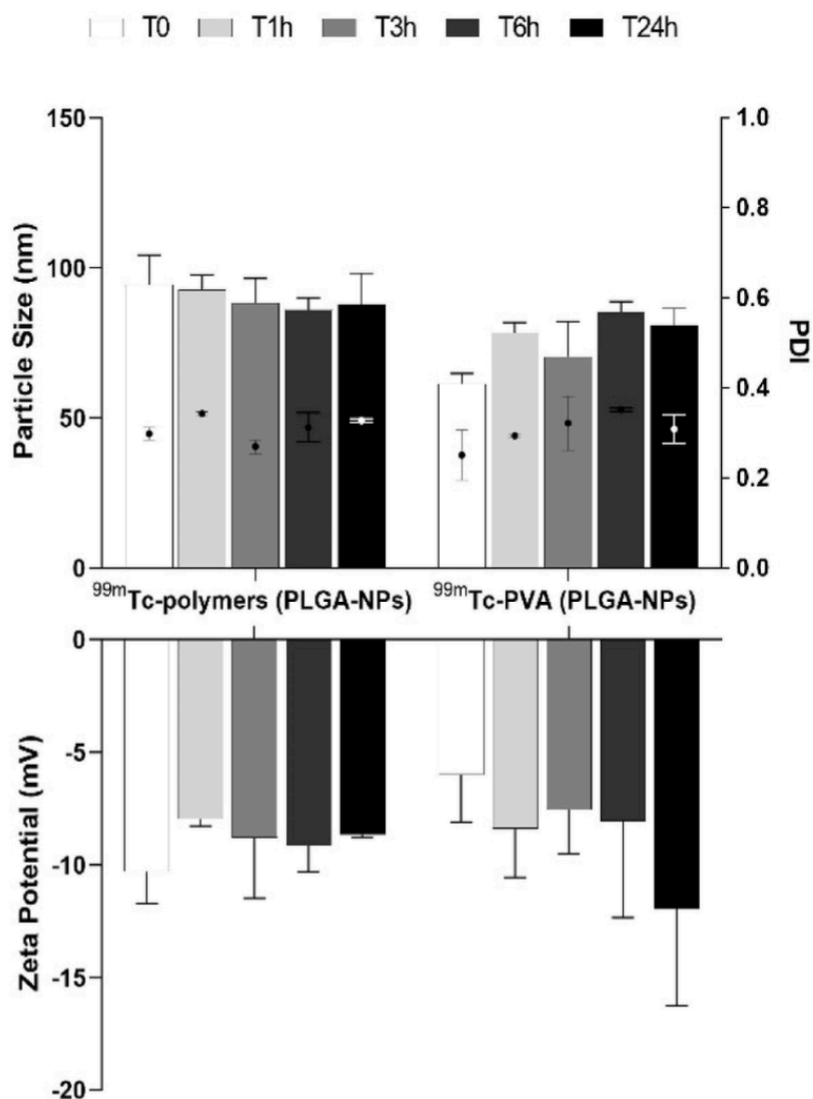
Figure 2. Particle size distribution and zeta potential measurements (bars) and PDI (dot) of batch #9 for both ^{99m}\text{Tc} -PVA (PLGA-NPs) and ^{99m}\text{Tc} -polymers (PLGA-NPs) at different time points (1, 3, 6, 24 h).
