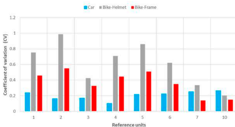
Figure 20. Coefficients of variations related to the a_{wz} values calculated in the sample units surveyed in bicycle and car during the field tests.
