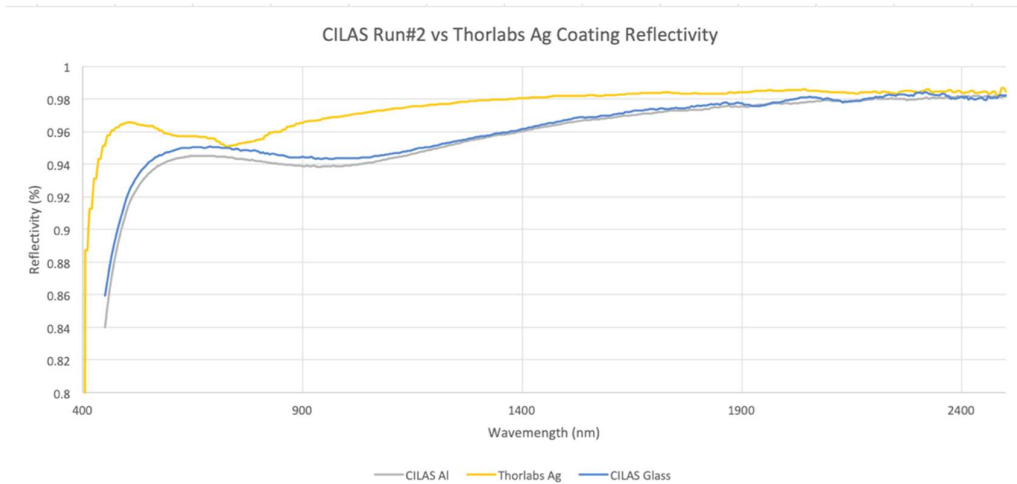
Figure 4. Protected-Ag coating measured reflectivity as compared to the expected reflectivity as reported by Thorlabs.
