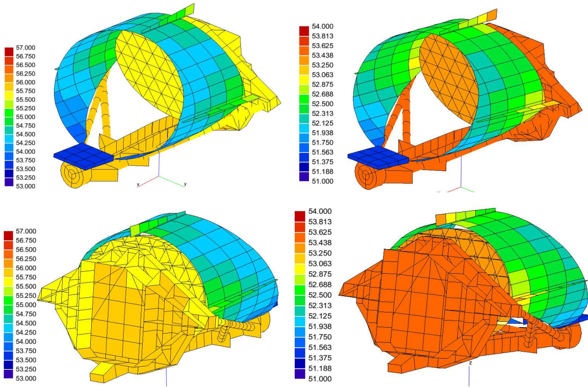
Figure 9. Views of the Telescope Assembly GTMM T map: Cold Case (left) and Hot Case (right).
