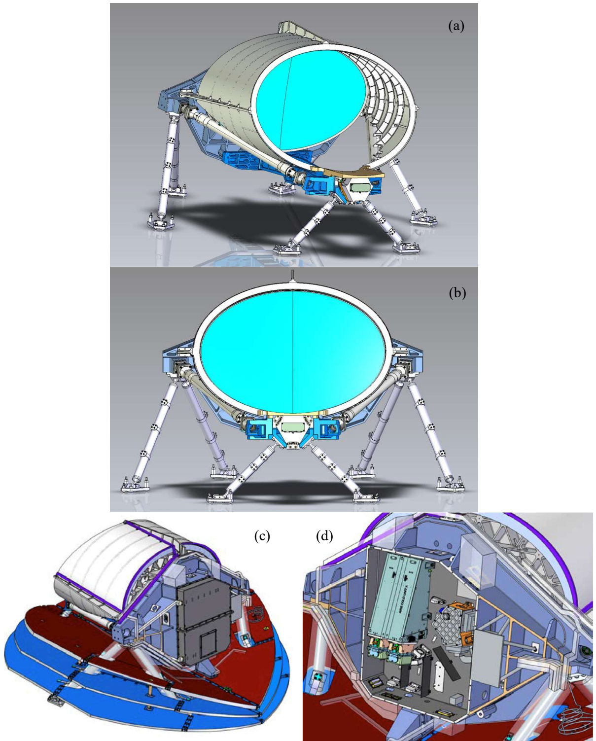
Figure 1. (a) Telescope assembly and bipods; (b) front view of the M1 mirror; (c) the Ariel payload showing the back of the telescope closed by the instrument radiator and the V-Grooves; (d) the optical bench and the instrument cavity.
