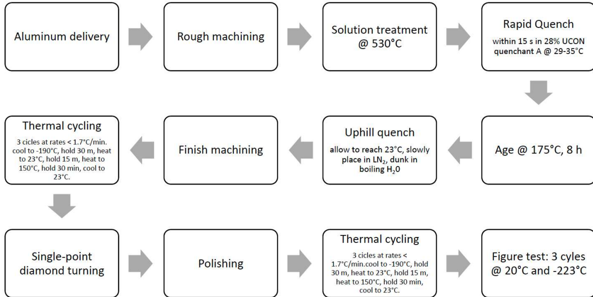
Figure 2. Manufacturing flow of the Ariel telescope mirrors based on Al 6061-T651
