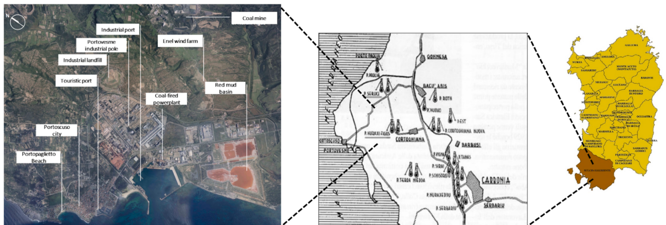
Fig. 3. From right to left: Localization of Sulcis territory in Sardinia, the Sulcis coal basin (Museo del carbone) and Portovesme industrial cluster. (adapted from Pessina, 2018 )
