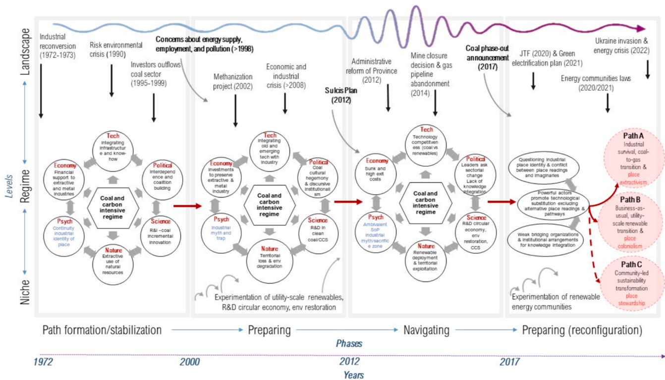
Fig. 4. Multi-level and multi-phase representation of Sulcis regime trajectory.
