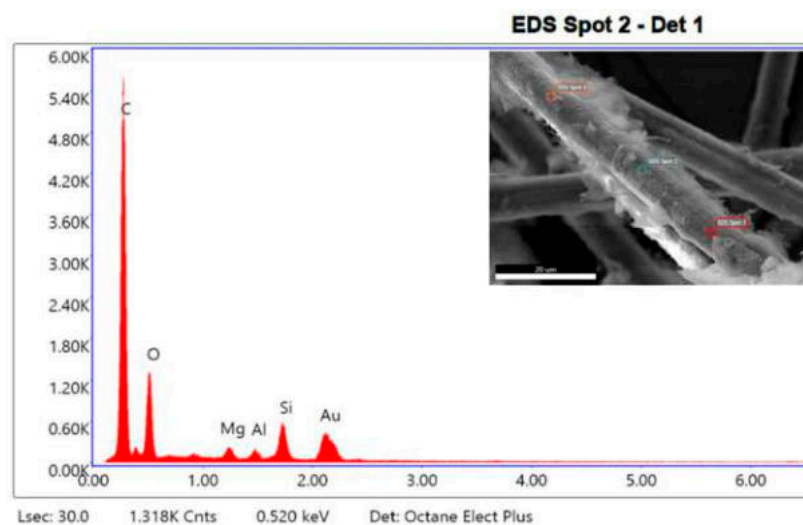
Figure 12. EDS spectrum of sCFs after conditioning with ANC.
