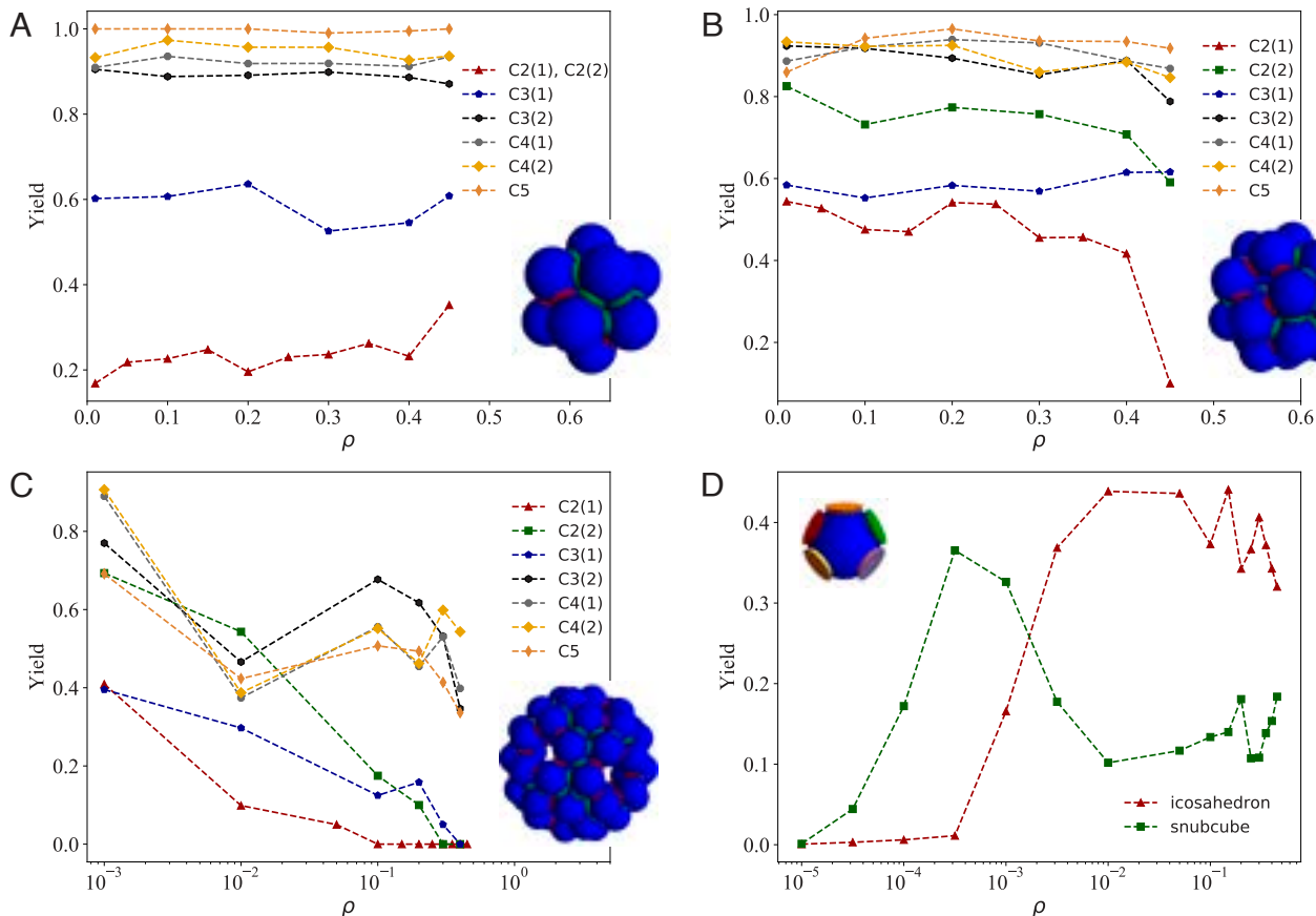
Fig. 4. Top: Graphic representation of the different one-component SAT solutions explored in this study, clarifying the respective patch coloring and interactions rules. Average yield of the icosahedron (A), snub cube (B), and snub dodecahedron (C) as a function of the density of patchy particles. These results were calculated with \cos \theta_{\max} = 0.98 and the in-plane angle, \gamma , was chosen to be the best for each structure. Thus, the icosahedron curve was calculated with \gamma = 60^\circ , the snub cube with \gamma = 90^\circ , and the snub dodecahedron with \gamma = 108^\circ . (D) shows the average yield as a function of density for the design of five colors, C5. Here, both curves were measured for the same system with \gamma = 85.45^\circ and \cos \theta_{\max} = 0.947 . All results shown in this figure were calculated at T = 0.097 . Temperature ( T ) is expressed in units of \epsilon and k_B = 1 , while all lengths are in units of \sigma .
