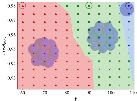
Fig. 3. Top: Snapshots of the final configurations obtained from simulations based on a one-component system (corresponding to the circles in the main diagram). Particles have two types of patches (red and green) and bind via self-complementary interactions (red with red and green with green). In all simulations, \cos\theta_{\max} = 0.98 and the \gamma = 60, 90 , and 108^\circ , respectively, i.e., at the optimal value for the three selected structures. The simulations for the icosahedron and snub cube were done with T = 0.097 and \rho = 0.01 , while for the snub dodecahedron, \rho = 0.001 was used. In all snapshots, the yield of the most probable shell is close to 100%. Bottom: Most probable structure formed for different in-plane angles, \gamma and for different patch width, \cos\theta_{\max} . The triangles inside the red region represent parameters where the most probable structure is the icosahedron. The squares inside the green region represent parameters where the most probable structure is the snub cube. The pentagons inside the blue region represent parameters where the most probable structure is the snub dodecahedron. Black crosses represent systems where only open/incomplete clusters are formed. The gray stars represent systems where clusters are able to close but none correspond to the ones in Fig. 1. Results were calculated for T = 0.097 and \rho = 0.01 . Temperature ( T ) is expressed in units of \epsilon and k_B = 1 , while all lengths are in units of \sigma .
