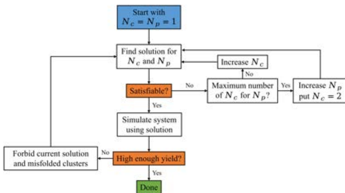
Fig. 8. Diagram of the SAT pipeline.
