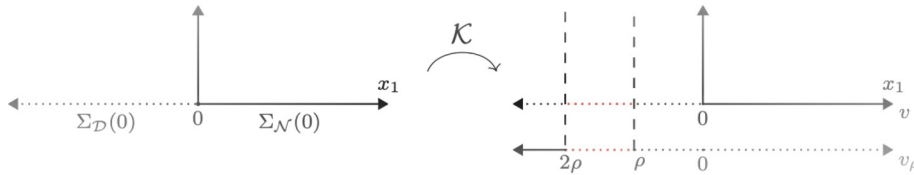
Fig. 2: The Kelvin transform centered at 0 acting on \Sigma_D(0) (dotted line) and \Sigma_N(0) for the functions v and v_\rho .
