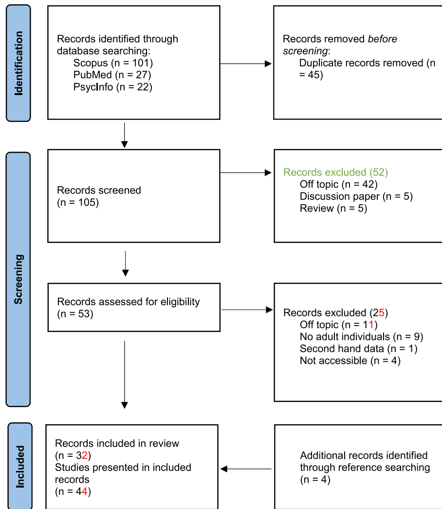
Fig. 1. Prisma flowchart.
