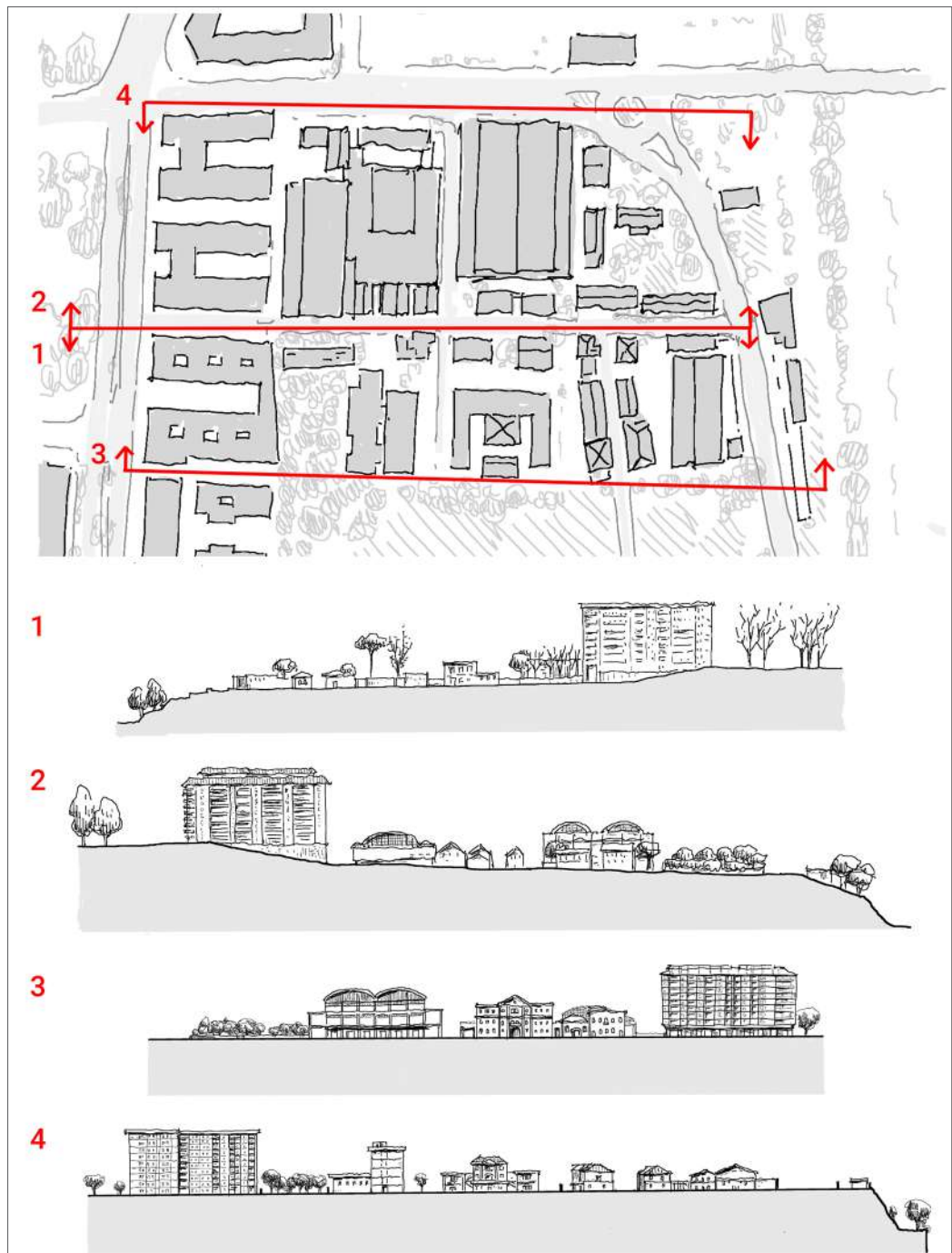
Fig. 03. Expeditious proportioning of the urban fronts of Via dei Papareschi, Via Pacinotti and the front behind Via Papareschi, with reference plan (elaboration of the authors).
