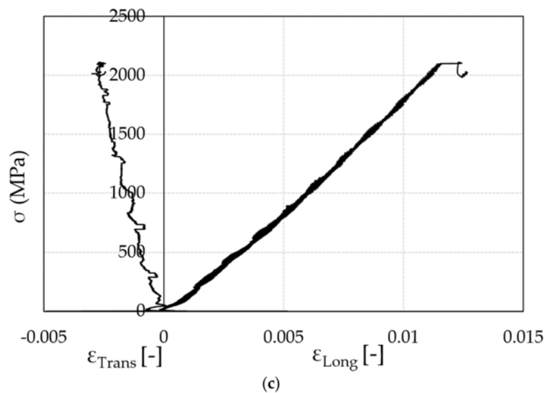
Figure 25. DIC analyses: (a) Left: undeformed mesh; Right: deformed mesh relative to a frame close to the cable break; (b) SA Specimen_3–Up: longitudinal strain distribution. The reported values have been obtained averaging the strain along the central alignment of the mesh (alignment 2 in Figure 18); (c) SA Specimen_3: experimental stress-strain curves (longitudinal –positive– and transversal –negative– strain).
