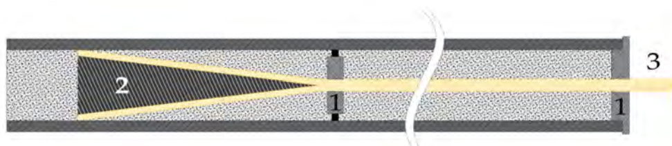
Figure 8. Spike anchorage proposed by Arnautov et al. [21]. In detail: 1—centering rings; 2—duralumin wedges; 3—rod.
