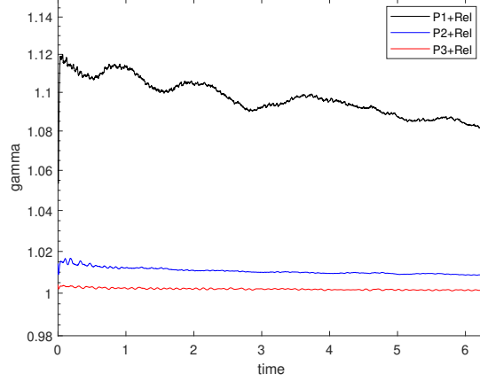
Figure 4: Values of \gamma^n for the rotating bump test case.
