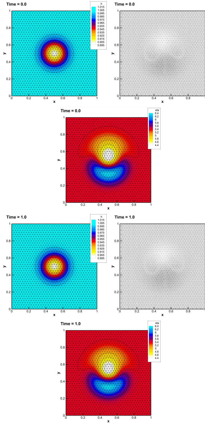
Figure 5: SW vortex test case. In the figure we report the profile of the density \rho (left), the velocity field (middle) and the entropy \eta (right) at time t = 0 (top row) and t = 1 (bottom row) obtained with a DG scheme of order 2 with relaxation on a coarse mesh made of 2840 elements.
