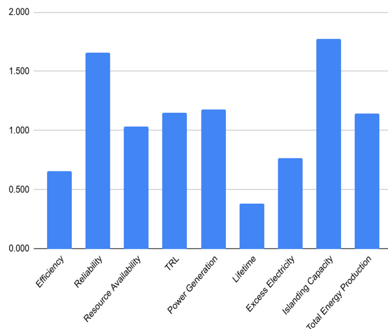
Figure 8. Average relative weight of technical criteria.
