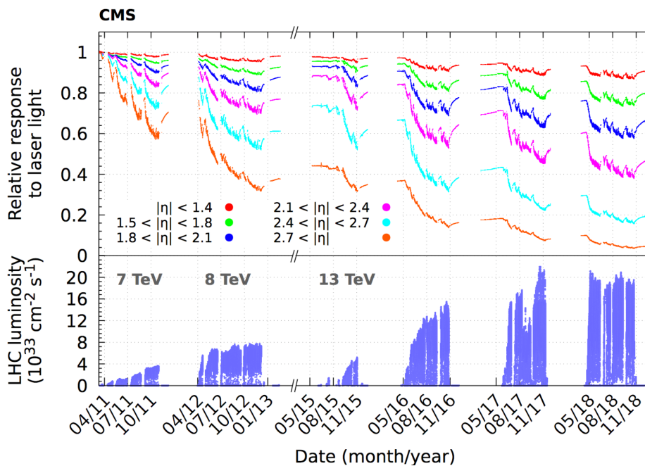
Figure 14. Relative response to laser light injected into the ECAL crystals, measured by the laser monitoring system, averaged over all crystals in bins of |\eta| . The response change observed in the ECAL channels is up to 13% in the barrel, |\eta| < 1.5 , and reaches up to 62% at |\eta| \approx 2.5 , the limit of the CMS inner tracker acceptance. The response change is up to 96% in the region closest to the beam pipe. The recovery of the crystal response during the periods without collisions is visible. These measurements, performed every 40 minutes, are used to correct the physics data. The lower panel shows the LHC instantaneous luminosity as a function of time.
