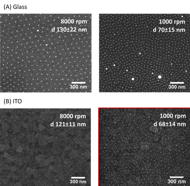
Fig. 2 Representative SEM images of (A) glass and (B) ITO substrates with AuNPs deposited by block-copolymer micellar lithography at two different spinning speeds, showing smaller average distances between gold particles ( d ), as the velocity decreases.
