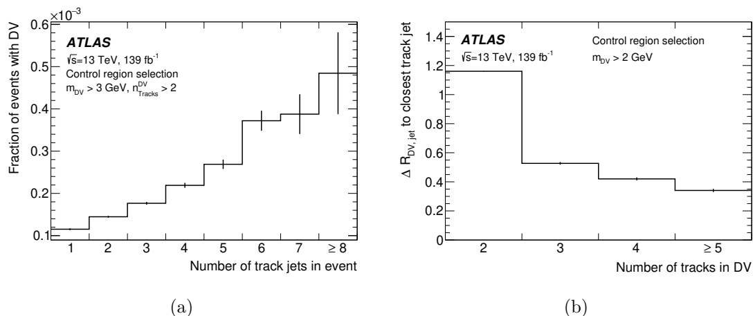
Figure 4. In (a), the fraction of events in the CR with a reconstructed DV satisfying m_{DV} > 3 GeV and n_{Tracks}^{DV} > 2 is shown. In (b), the average distance of DVs with m_{DV} > 2 GeV to the closest track jet in the event is shown, as a function of n_{Tracks} .
