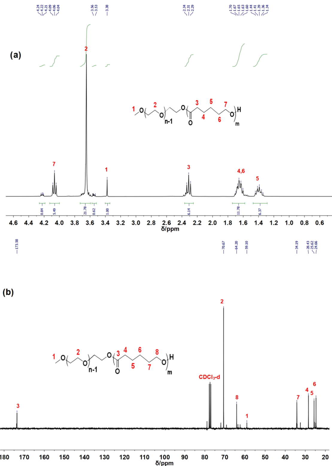
Figure 2. NMR characterization of MPEG- b -PCL diblock copolymer by using (a) 1 H NMR spectrum (CDCl 3 -d as a solvent, 400 MHz) and (b) 13 C NMR spectrum (CDCl 3 -d as a solvent, 150 MHz).
