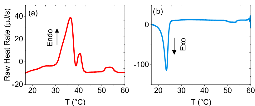
Figure 4. DSC heating (a) and cooling (b) curves of 1 wt % of MP(EG) 17 - b -P(CL) 9 in water. The heating and cooling rates were set at 0.2 °C/min.
