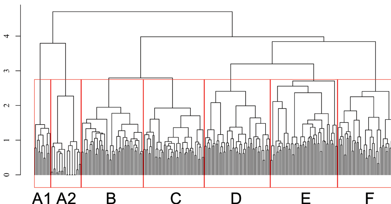
Figure 2. Dendrogram of relevés resulting from Ward's minimum variance clustering, with Euclidean distance as the similarity coefficient. Cluster A1 Corylus avellana forests. Cluster A2 Ostrya carpinifolia - Fagus sylvatica forests. Cluster B lower montane thermophytic Fagus sylvatica forests. Cluster C Middle montane, slightly acidic Fagus sylvatica forests. Cluster D upper montane basiphytic Fagus sylvatica forests. Cluster E middle montane basiphytic Fagus sylvatica forests. Cluster F upper-montane acidophytic Fagus sylvatica forests.
