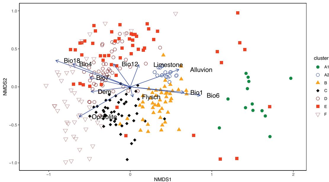
Figure 3. Non-Metric Multidimensional Scaling (NMDS) of relevés using Bray-Curtis dissimilarity index and a maximum of 20 random starts in search of the stable solution. Overlaid vectors represent the following environmental variables: Bio1: annual mean temperature; Bio4: Temperature Seasonality (standard deviation *100); Bio7: temperature annual range; Bio12: annual precipitation; Bio18: precipitation of warmest quarter; geological substrata include Ophiolite, Limestone, Flysch, Alluvion. Cluster A1 Corylus avellana forests. Cluster A2 Ostrya carpinifolia - Fagus sylvatica forests. Cluster B lower montane thermophytic Fagus sylvatica forests. Cluster C middle montane, slightly acidic Fagus sylvatica forests. Cluster D upper montane basiphytic Fagus sylvatica forests. Cluster E Middle montane basiphytic Fagus sylvatica forests. Cluster F Upper-montane acidophytic Fagus sylvatica forests.
