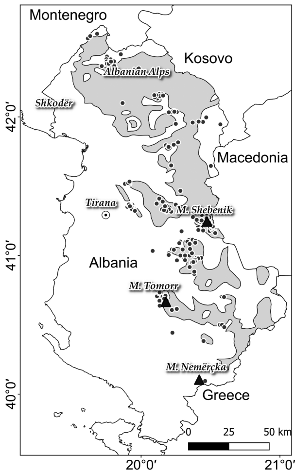
Figure 1. Study area. The black dots represent the relevés used in the analysis and the grey polygons represent the area of Fagus sylvatica forests according the Vegetation Map of Europe (Bohn et al. 2000, 2004).
