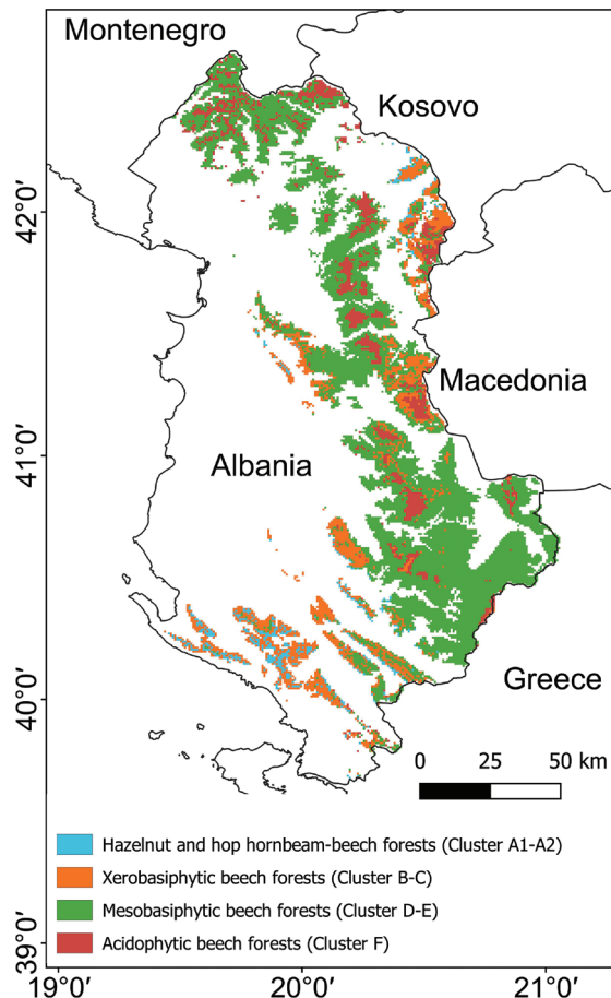
Figure 5. Map of the potential distribution of the four main groups of relevés resulting from random forest procedure. Cluster A1 Corylus avellana forests. Cluster A2 Ostrya carpinifolia-Fagus sylvatica forests. Cluster B lower montane thermophytic Fagus sylvatica forests. Cluster C middle montane, slightly acidic Fagus sylvatica forests. Cluster D upper montane basiphytic Fagus sylvatica forests. Cluster E middle montane basiphytic Fagus sylvatica forests. Cluster F upper-montane acidophytic Fagus sylvatica forests.
