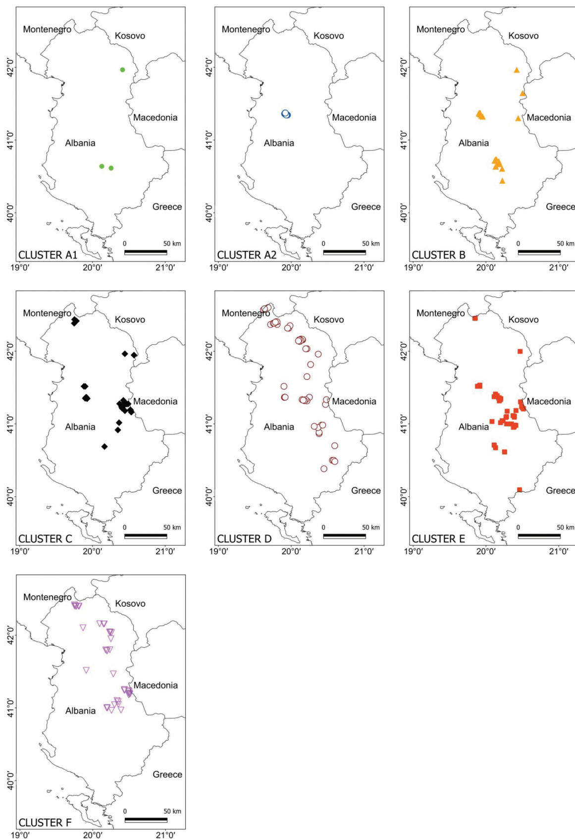
Figure 4. Distribution maps of the seven clusters of relevés. Symbols in the maps represent the sampling locations. Cluster A1 Corylus avellana forests. Cluster A2 Ostrya carpinifolia - Fagus sylvatica forests. Cluster B lower montane thermophytic Fagus sylvatica forests. Cluster C middle montane, slightly acidic Fagus sylvatica forests. Cluster D upper montane basiphytic Fagus sylvatica forests. Cluster E middle montane basiphytic Fagus sylvatica forests. Cluster F upper-montane acidophytic Fagus sylvatica forests.
