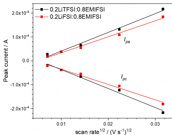
Figure 2. Linear fits for the anodic and cathodic peak currents versus square root of the scanning rates of a-Si electrodes using 0.2LiTFSI-0.8EMIFSI and 0.2LiFSI-0.8EMIFSI electrolytes. T = 20 °C.
