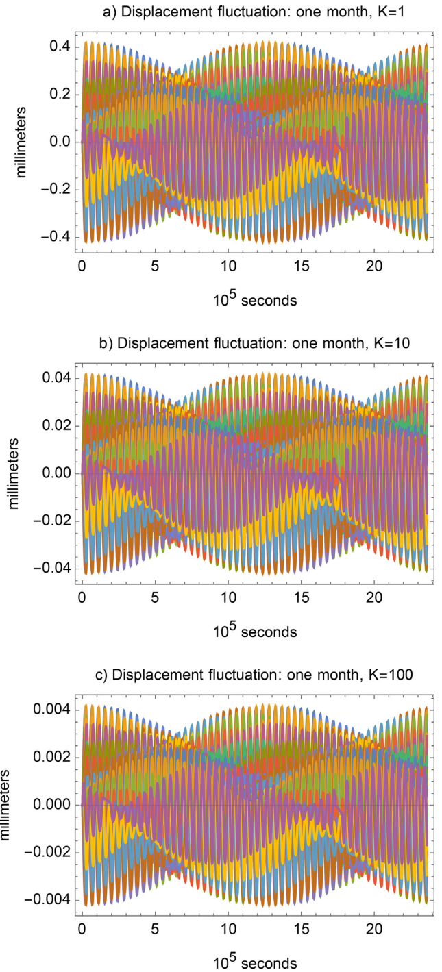
Fig. 4. Residual displacement around the linear trend for increasing values of K compared with \pm \frac{\omega_{m,s}t}{K} . We choose K = 1, 10, 100 \text{ s}^{-1} , corresponding to an effective shear viscosity of about \eta = 5 \times 10^{13}, 5 \times 10^{14}, 5 \times 10^{15} \text{ Pa}\cdot\text{s} .
