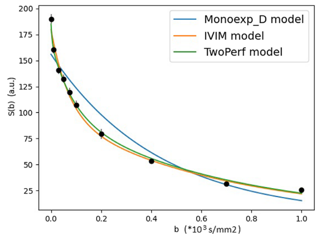
FIGURE 3: Example of a fit to DW-data obtained in the fetal ROI. The error bars were evaluated propagating the uncertainty on the noise \widehat{\sigma}_L^2 on the voxels inside the ROI. The Akaike weights are w_{\text{mono}}(\text{AIC}) = 6.2e-06 , w_{\text{IVIM}}(\text{AIC}) = 5.9e-2 , w_{2\text{perf}}(\text{AIC}) = 0.94 .
