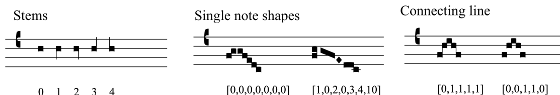
Illus. 14 Examples of elements modified at the single-note level: stems, individual note shapes and connecting line attributes, with corresponding encoded values assigned by the software. The value 0 represents the default and may also be empty. For single-note shapes, two ascending notes can form a pes shape (in which case the first note has a value of 1, while the second has 0 or no value). Two descending notes can form an oblique shape (where the first note has a value of 2, and the second has 0 or no value). Other values include punctum inclinatum (3), longa (4), and punctum with a ledger line (10)
