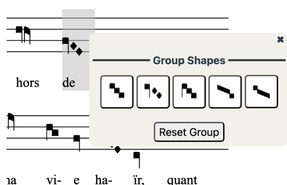
Illus. 12 Group shape menu for climacus
