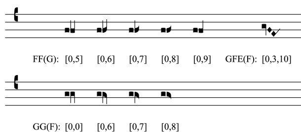
Illus. 15 Ligatures with final liquescence. MedMel character encoding (input by the user), indicates the notes, including the liquescent inflection, in round brackets, indicating the ascending or descending movements. In square brackets, the values associated to the single notes: in these cases, the first value is always 0 (or empty), the second value represent the notehead shape of the main note of the liquescent neume, while the note representing the liquescent inflection always has an empty value and it is thus not specified.
