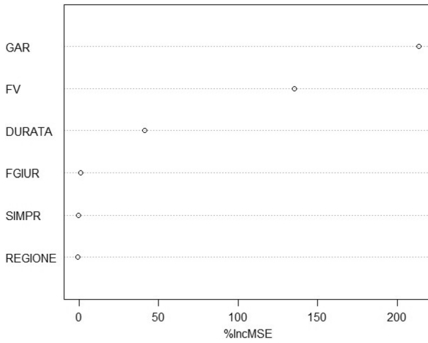
Fig. 2 Variable importance random forest
