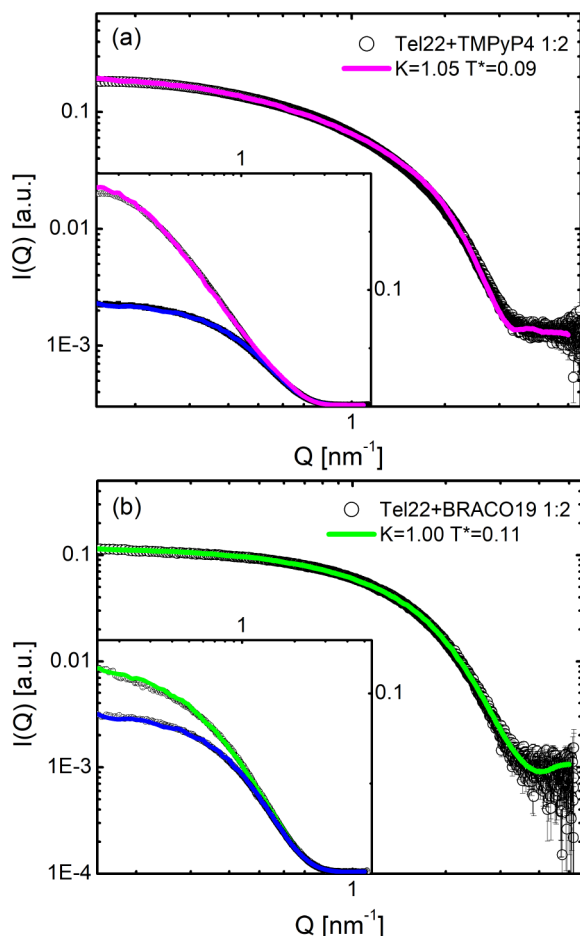
Figure 7. Experimental and simulated scattering intensities for Tel22+TMPyP4 (a) and Tel22+BRACO19 (b) solutions. Insets show in the semilogarithmic logscale the same curves together with the monomer profiles (blue lines).
