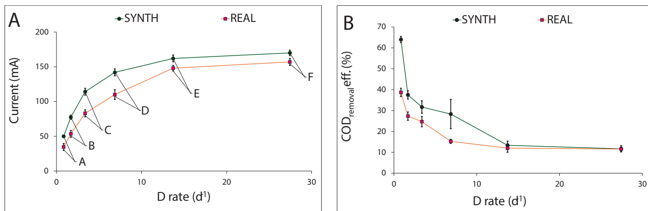
Fig. 2. Trends of the produced cathodic current (A) and of COD removal efficiency obtained (B) in MEC reactor as a function of D rate for all operating conditions, for both synthetic and real substrates.
