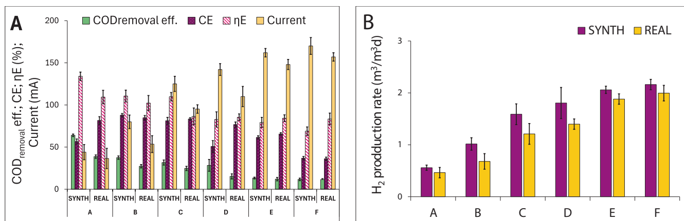
Fig. 3. Trends of the main characterizing parameters of the MEC system (A) and of the H 2 production rates (B) obtained for all operating conditions, for both synthetic and real substrates.
