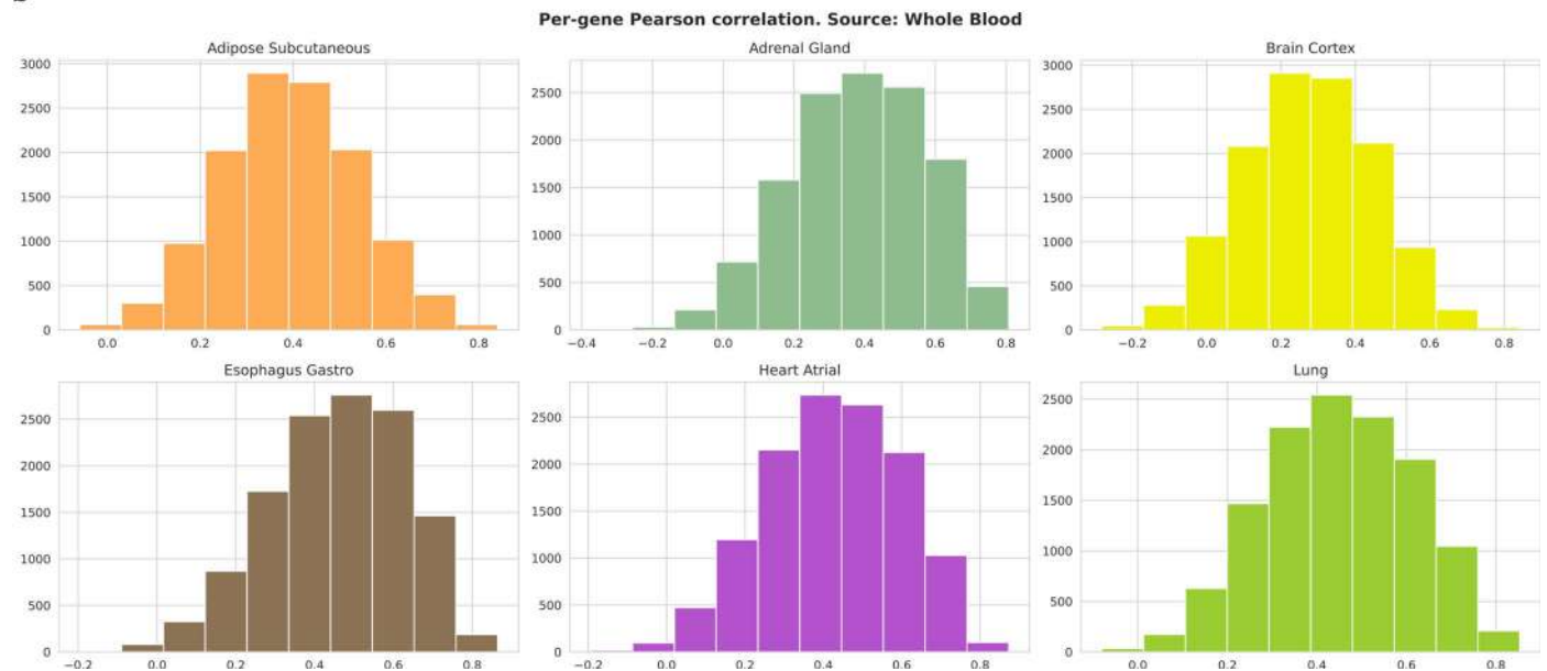
Extended Data Fig. 1 | Summary of per-gene prediction scores. (a) Network of tissues depicting the predictability of target tissues with HYFA using the average per-gene Pearson \rho correlation coefficients. Edges from reference to target tissues indicate an average per-gene \rho > 0.4 . The dimension of each node
