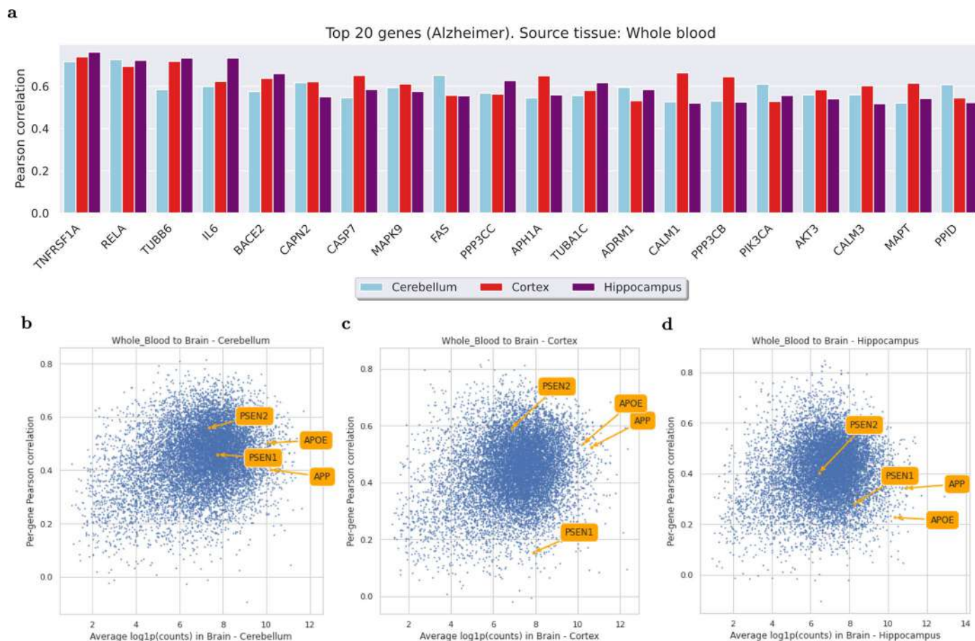
Extended Data Fig. 3 | Top predicted Alzheimer's disease-relevant genes in multiple brain regions, with whole blood as reference tissue. (a) Pearson correlation coefficient of top 20 predicted genes from the Alzheimer's disease pathway (KEGG), ranked by average correlation. (b, c, d) Average per-gene expression (x-axis) versus prediction performance (Pearson correlation between predicted and ground truth expression) in (b) cerebellum, (c) cortex, and (d) hippocampus. HYFA exhibits strong prediction performance for several
