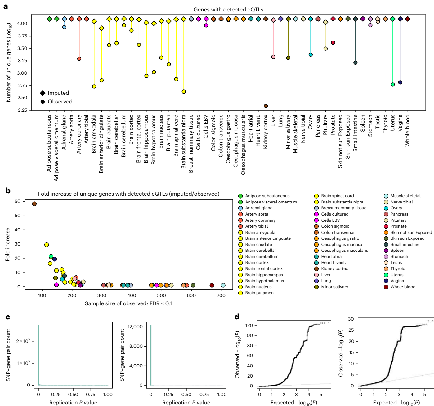
Fig. 5 | HYFA's imputed data improves eQTL discovery. a , Number of unique genes with detected eQTLs (FDR < 0.1) on observed (circle) and full (observed plus imputed; rhombus) GTEx data. Note logarithmic scale of y axis. The eQTLs were mapped using Matrix eQTL 55,70 assuming an additive genotype effect on gene expression. Matrix eQTL conducts a test for each single nucleotide polymorphism (SNP)–gene pair and makes adjustments for multiple comparisons by computing the Benjamini–Hochberg FDR 71 . b , Fold increase in number of unique genes with mapped eQTLs (y axis) versus observed sample size (x axis). c , Histogram of replication P values among the HYFA-identified cis-eQTLs
