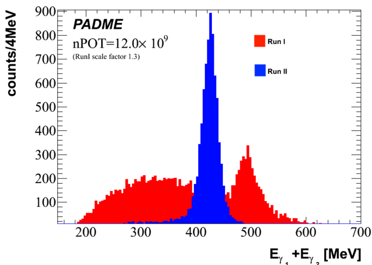
Figure 9. Total energy of cluster pairs during different running periods.
