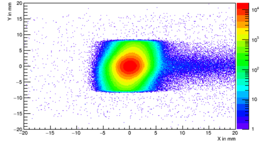
Figure 5. Beam spot at Flag 2 as seen from the ECal perspective. \sim 1000 bunch accumulated.
