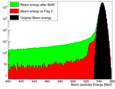
Figure 4. Beam energy profile as seen along different sections of the beam line.
