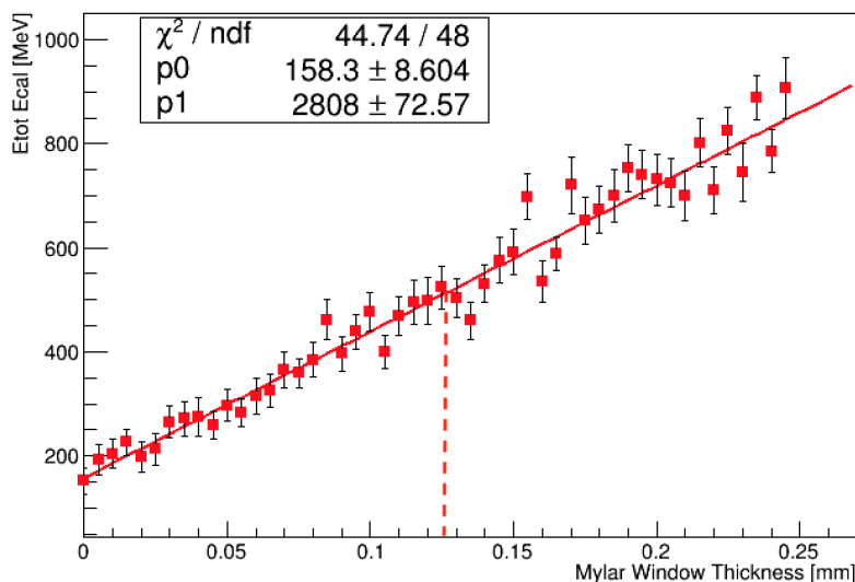
Figure 8. Impact of the window thickness on the PADME experiment background energy deposition for 25 \times 10^3 POT using the 2020 beam line configuration.
