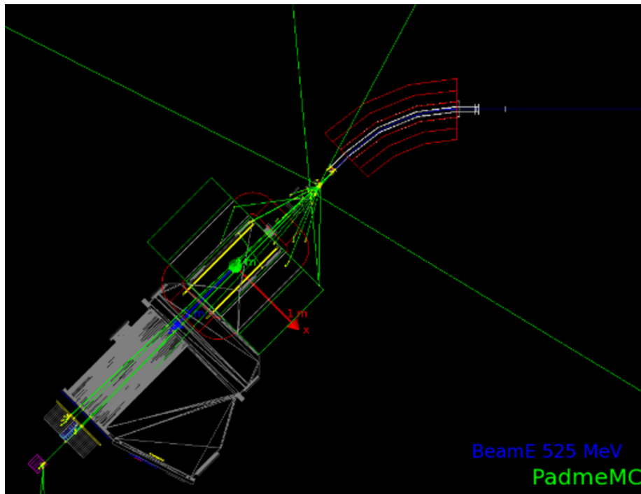
Figure 6. Low-energy positron striking the DHSTB002 dipole exit flange, thereby generating a shower. Green lines represent photons.
