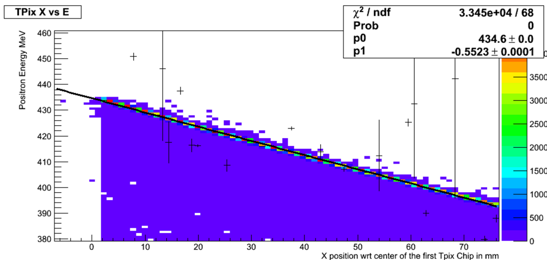
Figure 11. Calibration of the positron beam impact point on the TimePix detector with the MC simulation.
