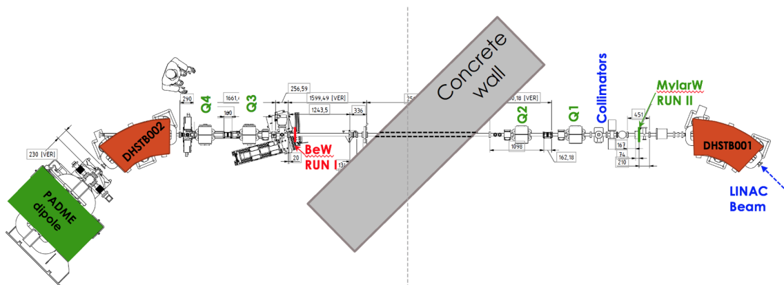
Figure 2. Drawing of the PADME beam line setup during Run II in 2020. Quoted dimensions are in mm.
