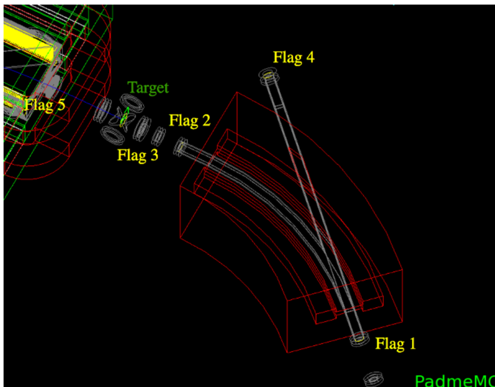
Figure 1. Detailed view of the PADME target region: in green Target with its support, in yellow the beam “Flags”, and in red the BTF DHSTB002 dipole magnet. On the top left side part of the PADME dipole magnet.
