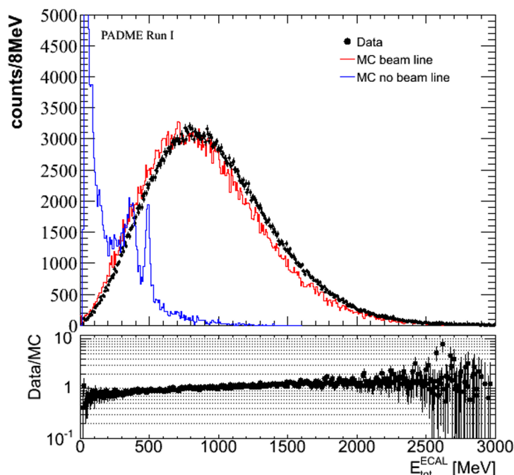
Figure 7. Total cluster energy distribution during Run I, measured experimentally (black dots), compared against MC simulation without beam transportation (blue line), and including beam transportation (red line). The bottom plot represents the ratio between data and simulation with beam transportation included.
