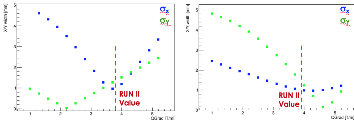
Figure 10. Beam transverse width on target vs. quadrupole Q3 (left) and Q4 (right). The vertical red-dashed line represents the actual gradient used during Run II.
