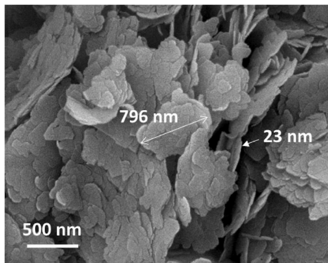
Fig. 4. Scanning electron micrograph of MWW(P)C sample.
