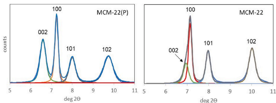
Fig. 2. Evolution of the XRD pattern of MCM-22(P) upon calcination, with decrease of the c cell parameter and formation of MCM-22.
