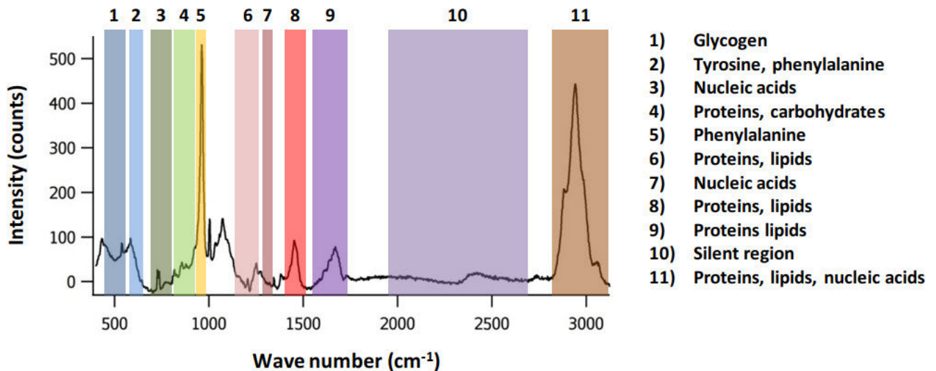
FIGURE 3. Example of a Raman spectrum of a biological sample, highlighting characteristic Raman bands and the related molecular assignment.
