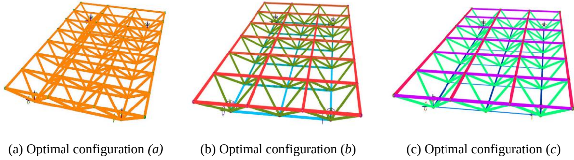
Fig. 5. 3D views of the optimized configurations for the three clustering strategies in Case Study 1.
