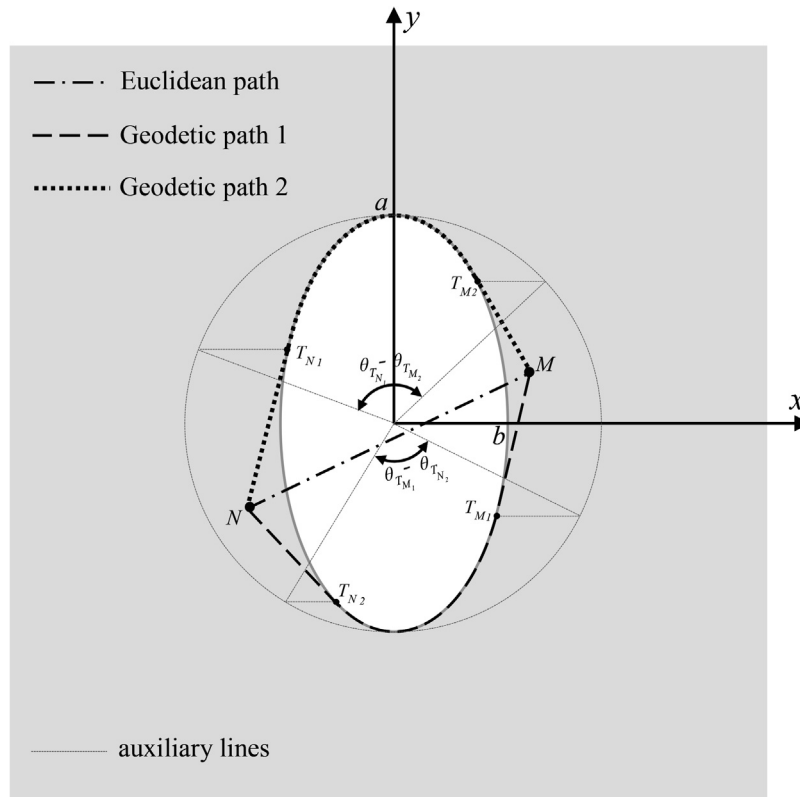
Fig. 1. Illustration of geodesic and Euclidean paths for points M and N .
