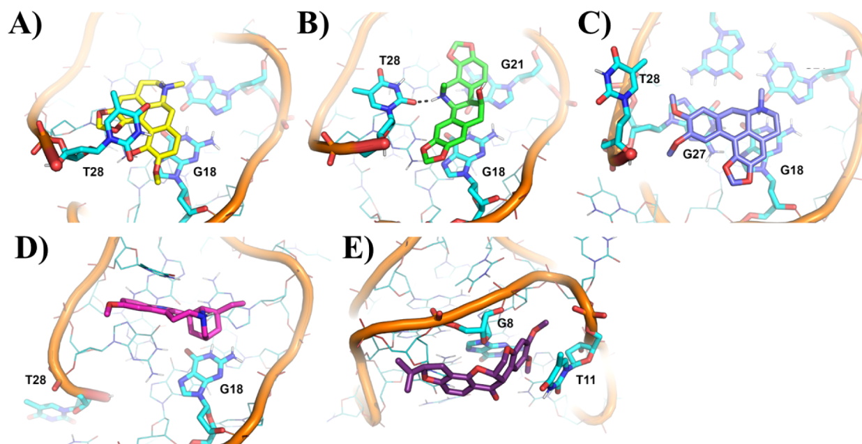
Figure 4. Binding mode of (A) bulbocapnine, (B) chelidoneine, (C) dicentrine, (D) ibogaine, and (E) rotenone to the AT11 G-quadruplex as obtained by MD simulations. The most representative frame extracted from the MD trajectories is shown. The natural compounds and the AT11 G-quadruplex are shown as sticks and ribbon, respectively. Bulbocapnine, chelidoneine, dicentrine, ibogaine, rotenone, and the AT11 G-quadruplex are colored in yellow, green, indigo, magenta, purple, and cyan, respectively. Polar interactions are shown by black dashed lines. Nucleotides involved in the interactions with the natural compounds are labeled and shown as sticks.
