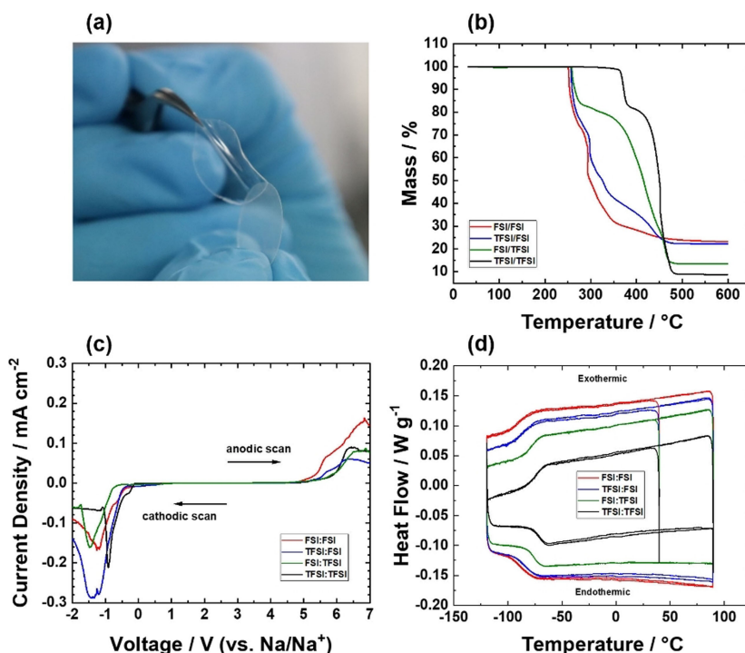
Figure 2. a) Photograph of the FSI:FSl SPE, b) TGA curves (heating rate of 5\text{ K min}^{-1} , inert \text{N}_2 atmosphere), c) anodic and cathodic LSV curves (Al foil as working electrode, Na metal as counter and reference electrode, scan rate of 0.1\text{ mV s}^{-1} ) and d) DSC curves (two cooling and heating cycles between -120\text{ }^\circ\text{C} and 90\text{ }^\circ\text{C} , cooling/heating rate of 5\text{ K min}^{-1} , 30 min isothermal holds at the turning points) of all four synthesized SPEs.
