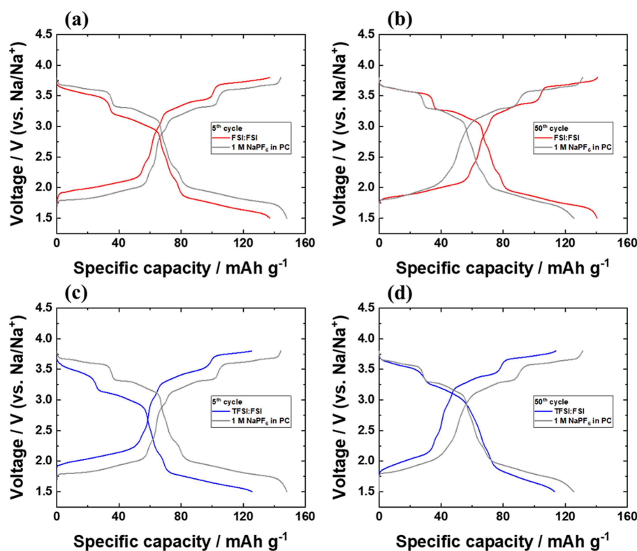
Figure 5. Voltage profiles of a, b) the FSI:FSI-based and c, d) TFSI:FSI-based SMB cell using NM as cathode in the 5 th and 50 th cycle (galvanostatic cycling with a current of 17 mA g -1 between 3.8 V and 1.5 V, temperature 20 °C \pm 2 °C). For comparison, the voltage profile in the carbonate-based liquid electrolyte is included.
