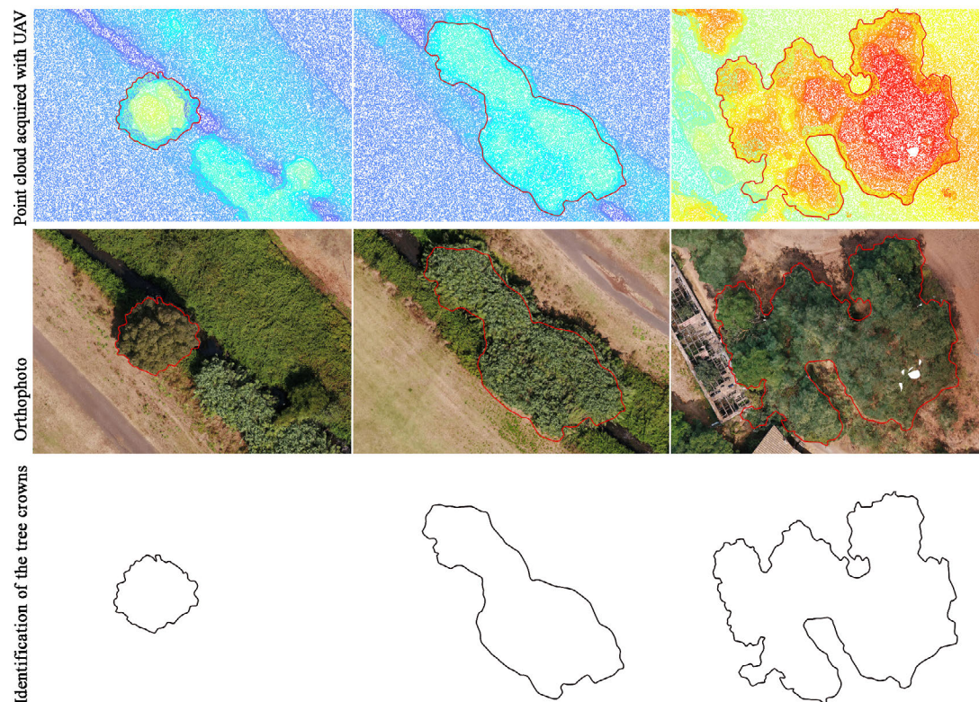
Fig. 13 - Identification of the crowns of the elements with punctual, linear and areal formation on the basis of the orthophoto derived from the point cloud and on the basis of the point cloud displayed using the elevation function (elaboration by the author in ESRI - ArcGIS Pro 2.7).
