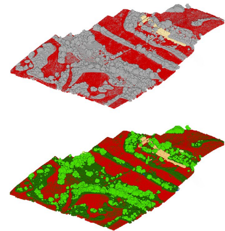
Fig. 9 - Classification of the point cloud in GIS (from top to bottom): Point cloud with unclassified RGB data; soil classification; building classification; and classification of plant elements (elaboration by the author in ESRI - ArcGIS Pro 2.7).
