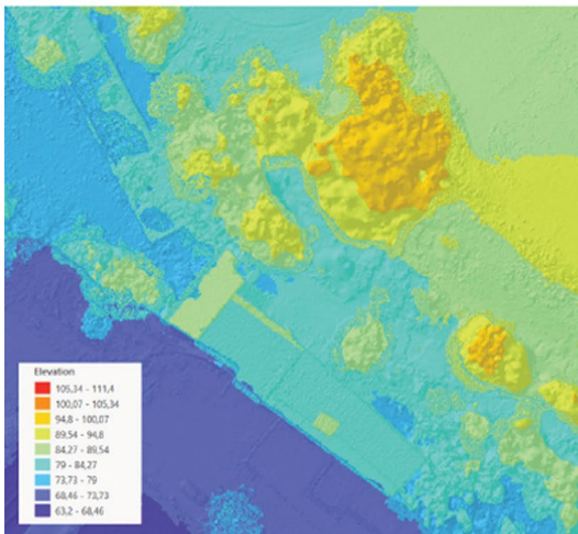
Fig. 7 - Top: Point cloud acquired with the UAV and imported into GIS, georeferenced, and displayed with RGB data. Bottom: Point cloud imported into GIS, georeferenced, and displayed with the surface draw method using the elevation function, which generates a visualisation with different coloured planes based on the elevation (elaboration by the author in ESRI - ArcGIS Pro 2.7).
