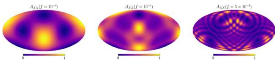
Fig. 40 Normalised auto-correlated response of TDI channel X at time t = 0 in the Solar System barycentre reference frame, at frequencies f = 10^{-4} Hz, f = 10^{-1} Hz, f = 5 \times 10^{-1} Hz from left to right respectively. Estimates based on (Contaldi et al. 2020)
