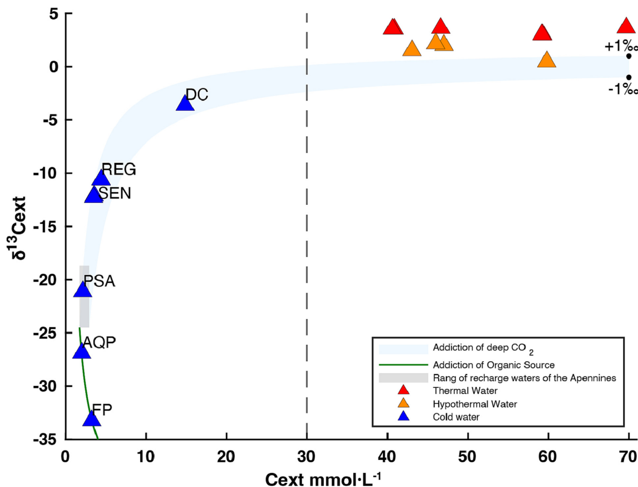
Fig. 5. C_{ext} vs. \delta^{13}C_{ext} diagram. The theoretical field resulting from the addition of C_{deep} with \delta^{13}C_{deep} ranging from -1 to +1 \text{ ‰} to infiltrating water with C_{inf} = 2.31 \pm 0.61 \text{ mmol} \cdot L^{-1} and \delta^{13}C_{inf} = -21.6 \pm 2.9 \text{ ‰} is indicated in Fron dini et al., 2019. The green line represents the theoretical mixing between the infiltrating water and an organic source. The dashed vertical line represents the C_{ext} upper limit for the applicability of the no-sink assumption.
