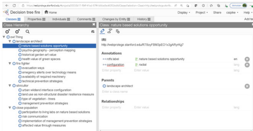
Fig. 4 Decision ontology a multihazard ontology, b surroundings
