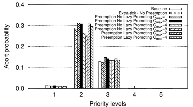
Figure 7. Variation of the transaction abort probability.
