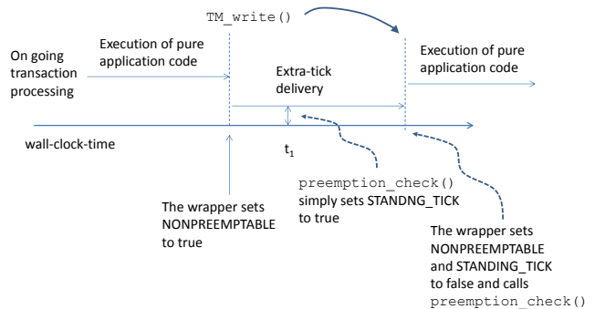
Figure 4. Standing ticks and time shift of preemptions.
