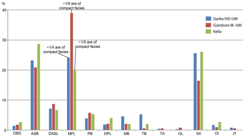
Fig. 6 - Lithological composition of the ancient alluvial deposits approximately dated to 1.5 Ma. ASB: aphyric to subaphyric basalt; DASL: differentiated aphyric to subaphyric lavas; DPL: differentiated porphyritic lavas; IT: ignimbritic tuff; MB: microdoleritic basalt; MFL: Melka Fault lava; OBS: obsidian; OI: other types of welded ignimbrite; OL: obsidian lava; PB: porphyritic basalt; TA: trachyandesite; TB: trachybasalt; WI: welded ignimbrite no. 1. The colour version of this figure is available at the JASs website.
