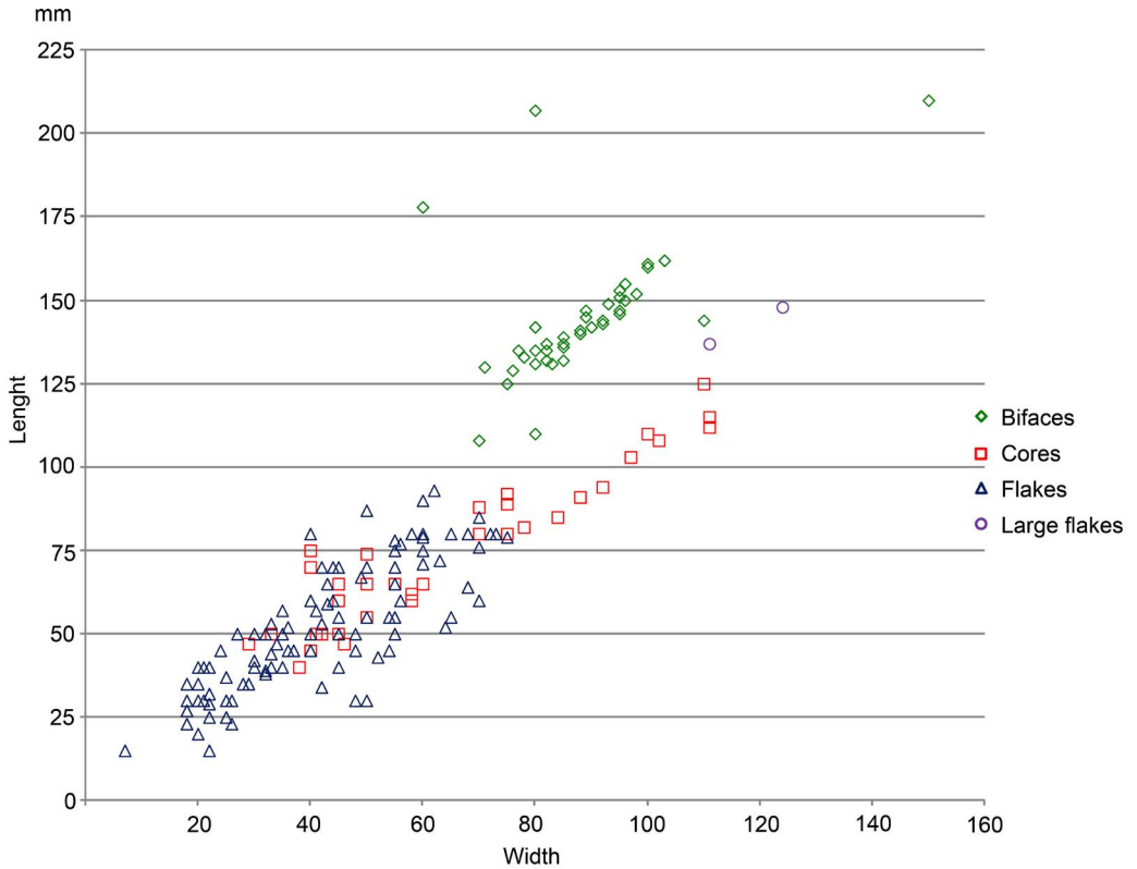
Fig. 10 - Gombore II OAM. Size distribution (mm) of the artifacts analyzed in this paper. The colour version of this figure is available at the JASs website.
