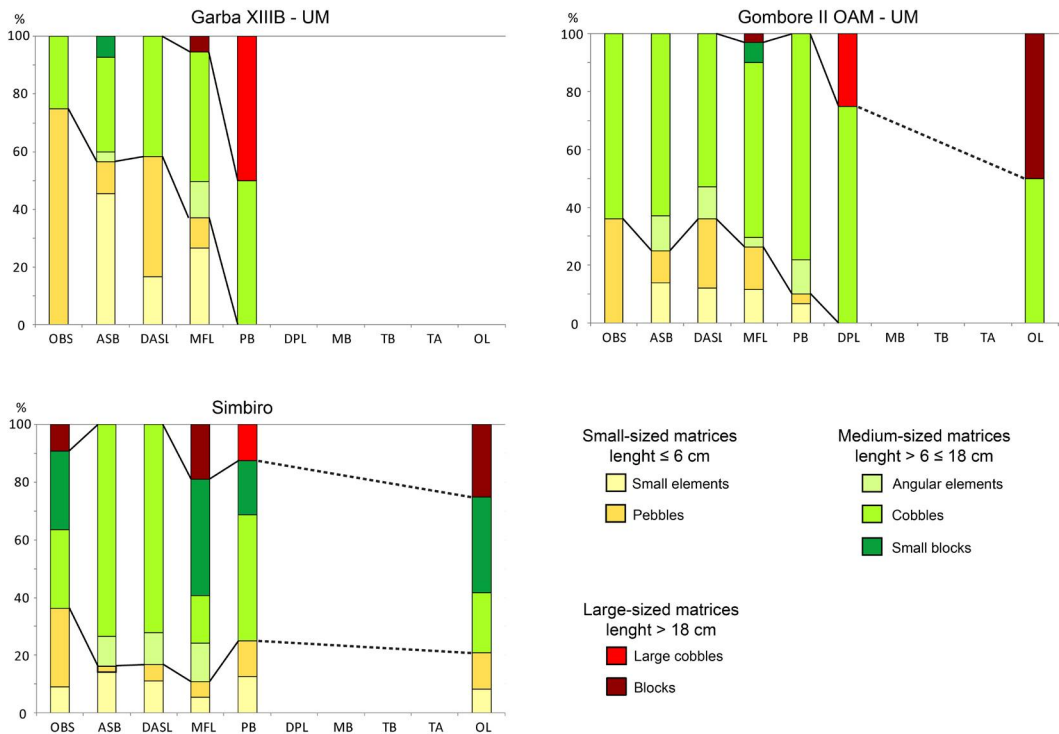
Fig. 9 - Frequencies of morphometric types in alluvial deposits approximately dated to 1.0-0.85 Ma. Welded ignimbrite no. 1, other types of welded ignimbrite and ignimbritic tuff are not shown because they were never used for knapping. ASB: aphyric to subaphyric basalt; DASL: differentiated aphyric to subaphyric lavas; DPL: differentiated porphyritic lavas; MB: microdoleritic basalt; MFL: Melka Fault lava; OBS: obsidian; OL: obsidian lava; PB: porphyritic basalt; TA: trachyandesite; TB: trachybasalt. The colour version of this figure is available at the JASS website.
