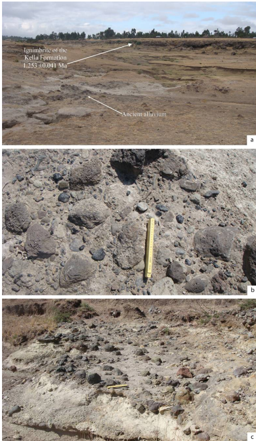
Fig. 5 - Sampled ancient alluvial deposits: (a) Kella; (b) detail of Kella; (c) Simbiro. The colour version of this figure is available at the JAS website.
