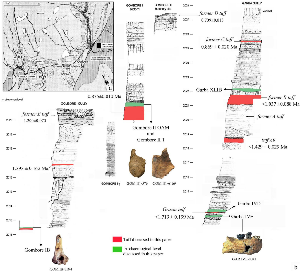
Fig. 2 - (a) Geological sketch map of the Melka Kunture area (after Taieb, 1974, revised); (b) the Melka Kunture Formation, showing the location of the archeological levels and human fossils discussed in this paper (after Raynal et al., 2004, revised; radiometric dates after Morgan et al., 2012). The colour version of this figure is available at the JASS website.
