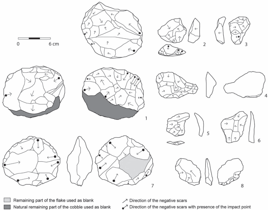
Fig. 17 - Garba XIII B. Small débitage cores and flakes. 1: multifacial multidirectional irregular core; 2, 3: flakes from multifacial exploitation; 4-6, 8: flakes from discoid exploitation; 7: bifacial discoid core on flake. Aphyric basalt (after Gallotti et al. , 2014).
