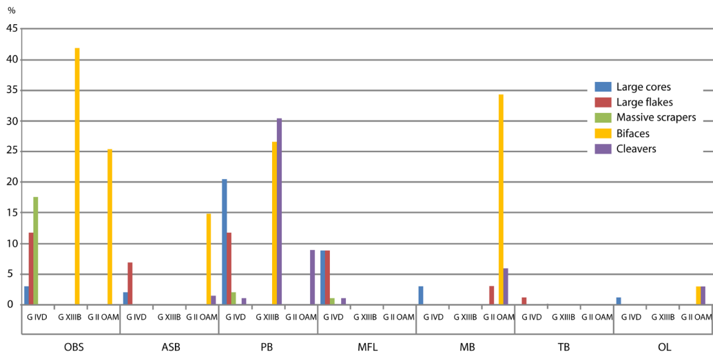
Fig. 13 - Lithological composition and technological components of the LCT productions at Garba IVD (G IVD), Garba XIIIIB (G XIIIIB) and Gombore II OAM (G II OAM). ASB: aphyric to subaphyric basalt; MB: microdoleritic basalt; MFL: Melka Fault lava; OBS: obsidian; OL: obsidian lava; PB: porphyritic basalt; TB: trachybasalt. Twisted bifaces are not included because they constitute unique discovery not only at Melka Kunture, but also in East Africa. The colour version of this figure is available at the JASs website.
