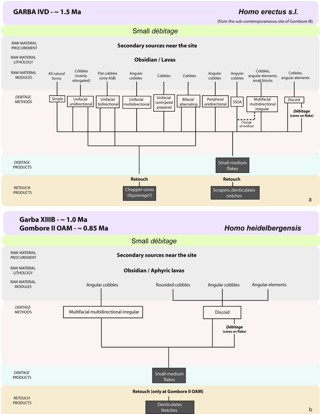
Fig. 21 - Schematic reconstruction of small-medium flake productions and associated hominins at Garba IVD (a), Garba XIII B, and Gombore II OAM (b). The colour version of this figure is available at the JASs website.
