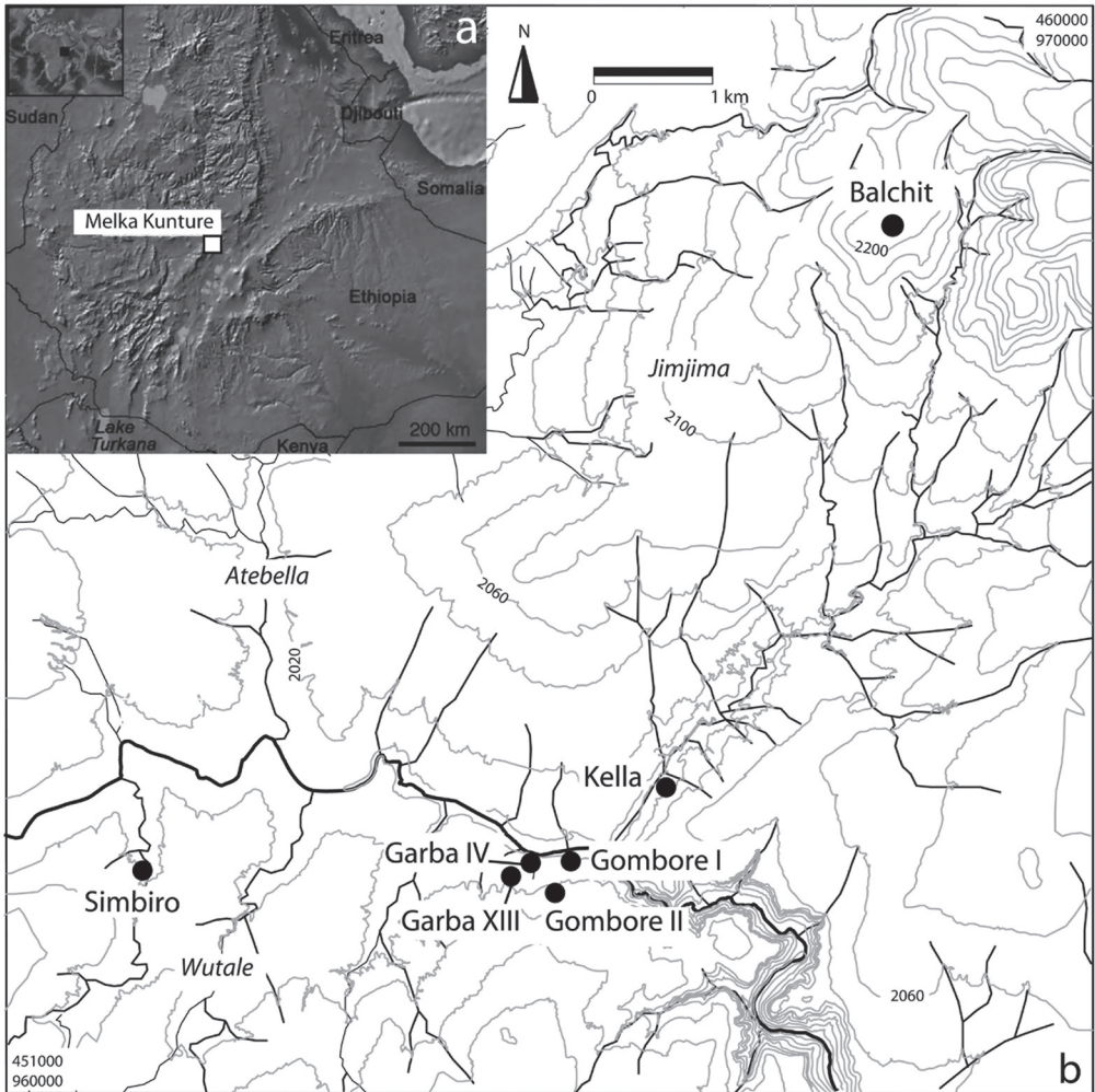
Fig. 1 - (a) Location of Melka Kunture on the shoulder of the Main Ethiopian Rift; (b) Map of the Melka Kunture area showing the location of archeological sites, of old alluvial deposits, and of raw material primary sources (vector restitution of the 1:50,000 topographic map). The primary sources of aphyric lavas and microdoleritic basalts are outside the area: aphyric lavas are among the pre-rift lava flows of Addis Ababa and Guraghe-Anchar basalts, respectively 26 km N-E and 45 km S-W of Melka Kunture (Abebe et al., 2005), whereas microdoleritic basalts outcrop closer, 15-20 km north and south of Melka Kunture.
