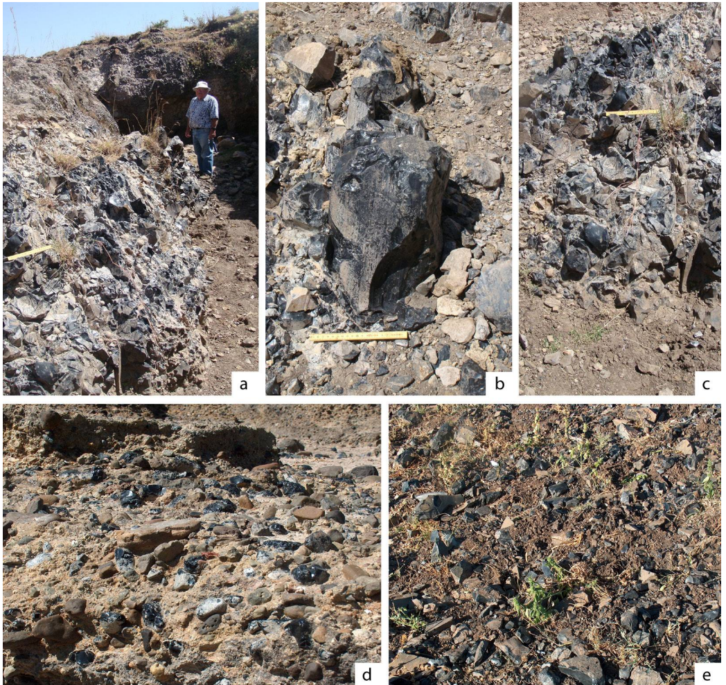
Fig. 4 - (a) Obsidian outcrop at Balchit; (b-c) obsidian blocks among weathered rocks; (d) obsidian cobbles and gravels in an ancient alluvium at Atebella; (e) obsidian angular elements on the ground at Balchit. The colour version of this figure is available at the JASs website.
