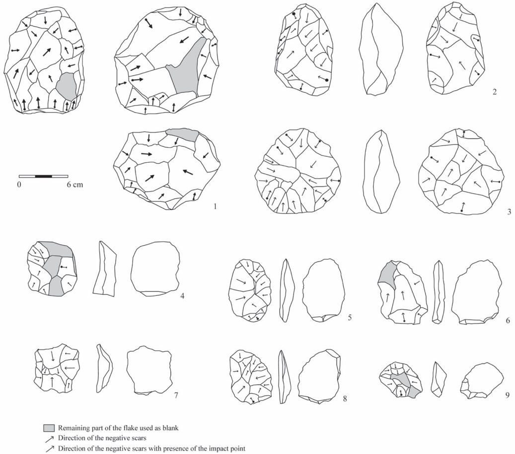
Fig. 12 - Gombore II OAM. Cores and flakes from small débitage. 1: multifacial multidirectional core; 2, 3: bifacial discoid cores; 4, 7: flakes from multifacial exploitation; 5, 6, 8, 9: flakes from discoid exploitation. 1, 3-6: aphyric basalt; 2, 7-9: obsidian.
