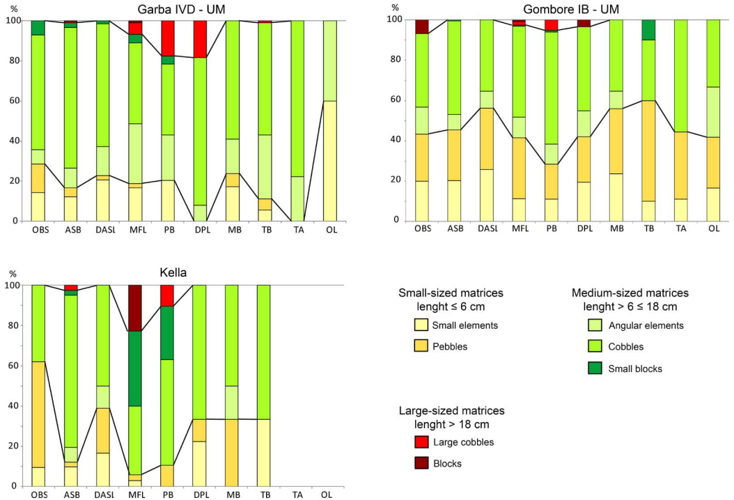
Fig. 7 - Frequencies of morphometric types in alluvial deposits approximately dated to 1.5 Ma. Welded ignimbrite no. 1, other types of welded ignimbrite and ignimbritic tuff are not shown because they were never used for knapping. ASB: aphyric to subaphyric basalt; DASL: differentiated aphyric to subaphyric lavas; DPL: differentiated porphyritic lavas; MB: microdoleritic basalt; MFL: Melka Fault lava; OBS: obsidian; OL: obsidian lava; PB: porphyritic basalt; TA: trachyandesite; TB: trachybasalt. The colour version of this figure is available at the JASs website.
