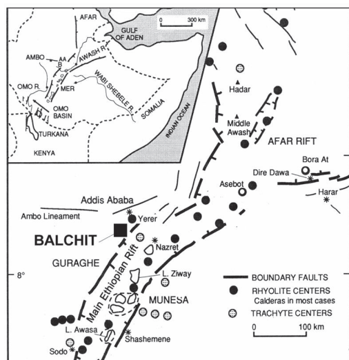
Fig. 3. Map showing the location of the Balchit and other obsidian outcrops (after WoldeGabriel et al. , 1992, revised).
