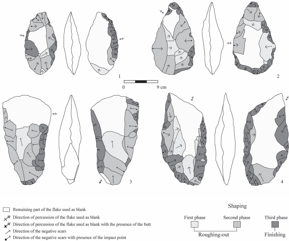
Fig. 15 - Garba XIII B. Bifaces (1, 2) and cleavers (3, 4) on Kombewa flake blanks of porphyritic basalt.
