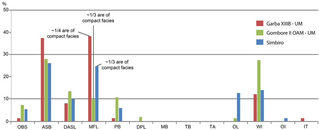
Fig. 8 - Lithological composition of ancient alluvial deposits approximately dated to 1.0-0.85 Ma. ASB: aphyric to subaphyric basalt; DASL: differentiated aphyric to subaphyric lavas; DPL: differentiated porphyritic lavas; IT: ignimbritic tuff; MB: microdoleritic basalt; MFL: Melka Fault lava; OBS: obsidian; OI: other types of welded ignimbrite; OL: obsidian lava; PB: porphyritic basalt; TA: trachyandesite; TB: trachybasalt; WI: welded ignimbrite no. 1. The colour version of this figure is available at the JASs website.
