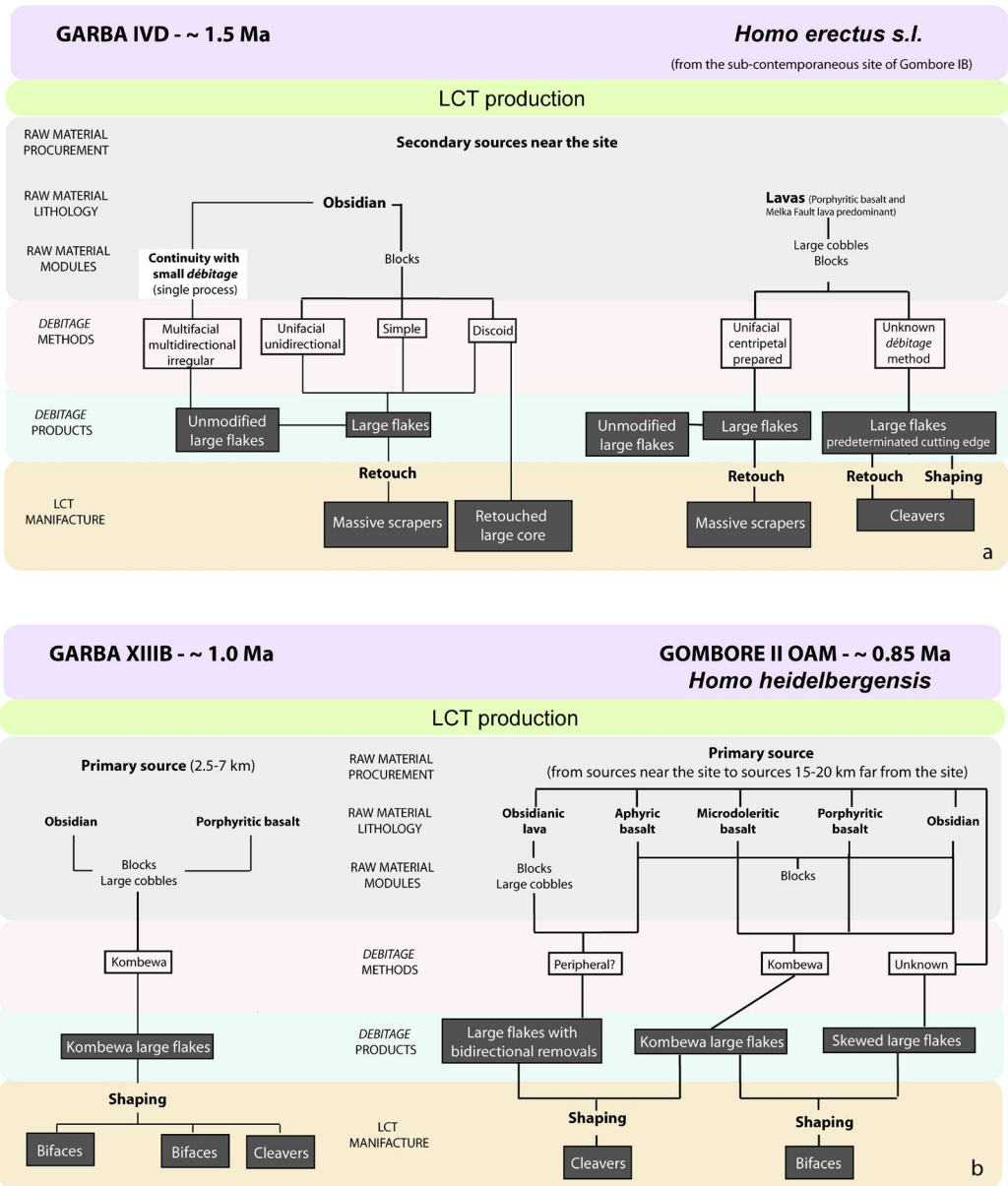
Fig. 20 - Schematic reconstruction of LCT productions and associated hominins at Garba IVD (a), Garba XIII B, and Gombore II OAM (b). The colour version of this figure is available at the JASs website.
