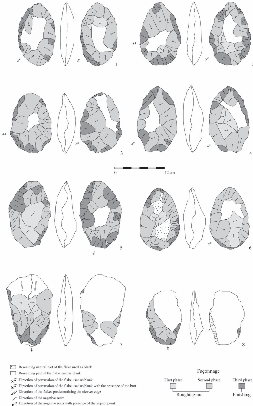
Fig. 11 - Gombore II OAM. Bifaces and cleavers. 1-4: bifaces on Kombewa flakes. 5, 6: bifaces on skewed flakes; 7: cleaver on flake with bidirectional removals; 8: cleaver on Kombewa flake. 1, 2, 4, 5, 8: microdoleritic basalt; 3: obsidian; 6: aphyric basalt; 7: obsidian lava. 1, 6-8 after Gallotti et al., 2010.
