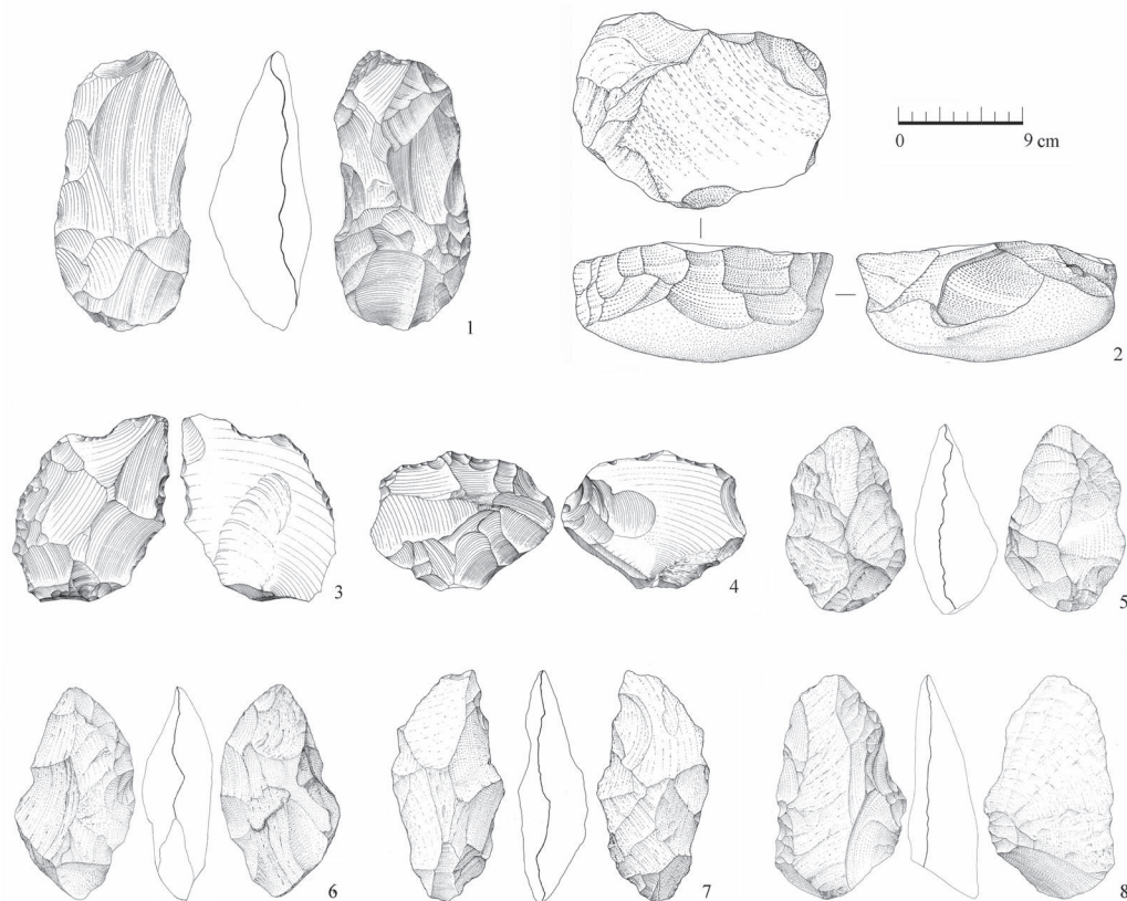
Fig. 14 - LCT production at Garba IVD. 1: discoïd core; 2: unifacial centripetal prepared core; 3-6: massive scrapers; 7-8: cleavers. 1, 3, 4: obsidian; 2, 7: Melka Fault lava; 5, 6, 8: porphyritic basalt. Drawings by M. Pennacchioni; after Gallotti, 2013.
