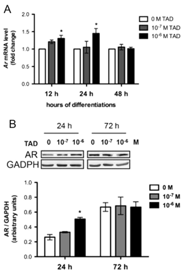
Fig. 4 Effects of TAD ( 10^{-7} to 10^{-6} M) on a) AR mRNA expression levels after 12, 24, and 48 h the onset of differentiation; b) AR protein expression after 24 and 72 h of differentiation. * p \leq 0.05 vs. untreated cells
