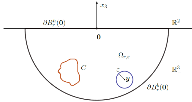
FIGURE 3.1. Domain \Omega_{r,\varepsilon} .
