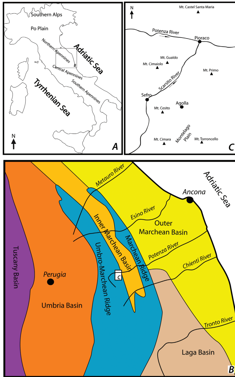
Fig. 1 - Location of the study area in the UMS Basin (after Fabbi, 2015).
