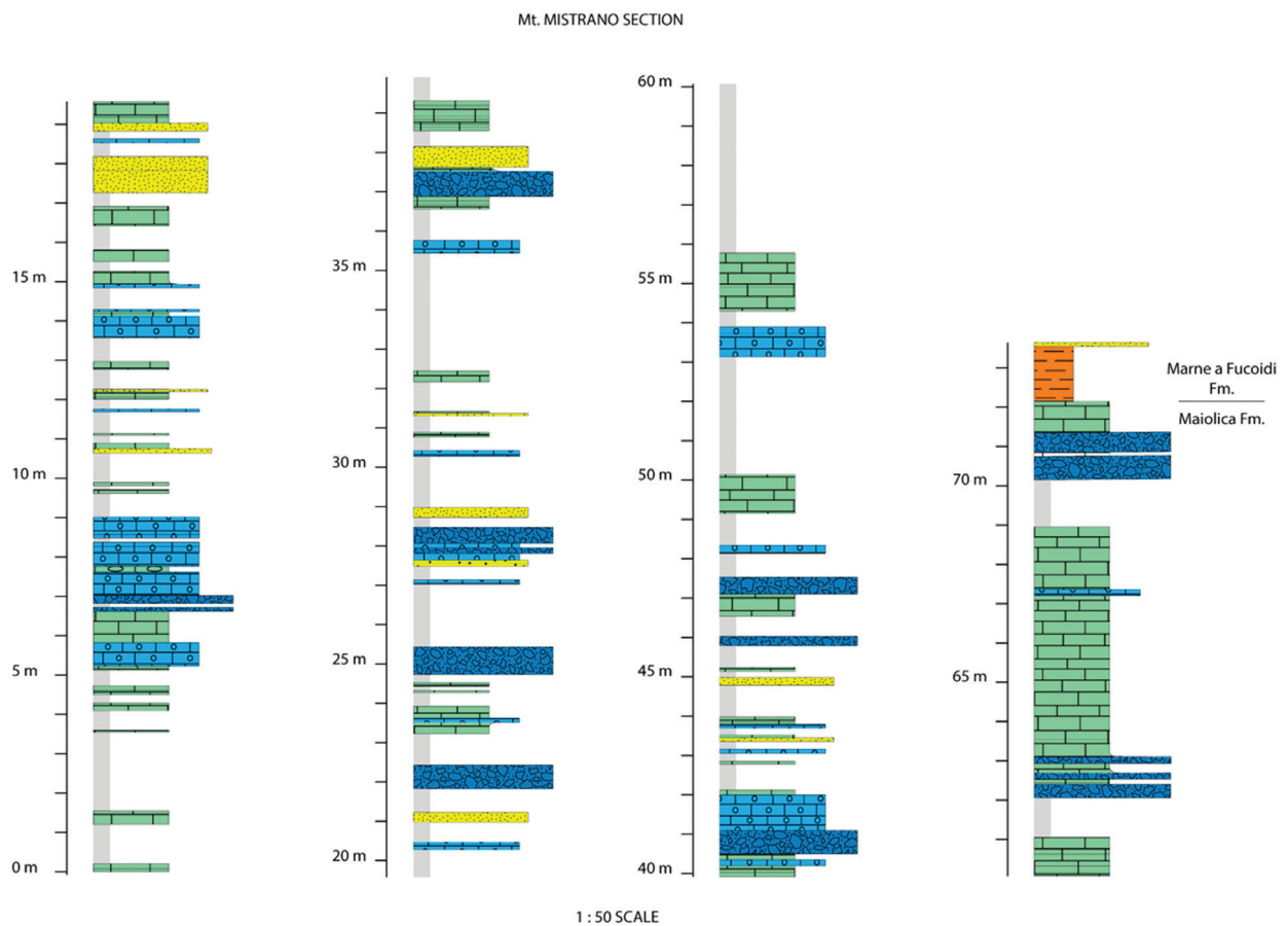
Fig. 10 - The Mt. Mistrano section stratigraphic log. See Fig. 9 for legend.
