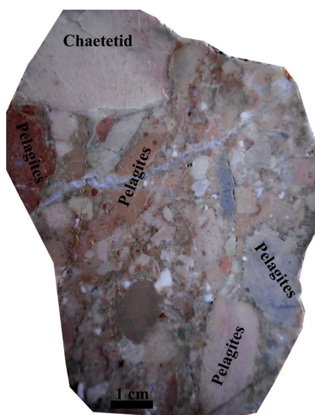
Fig. 11 - Polished slab of a calcirudite with clasts of condensed pelagites and chaetetids (Mt. Mistrano section).
