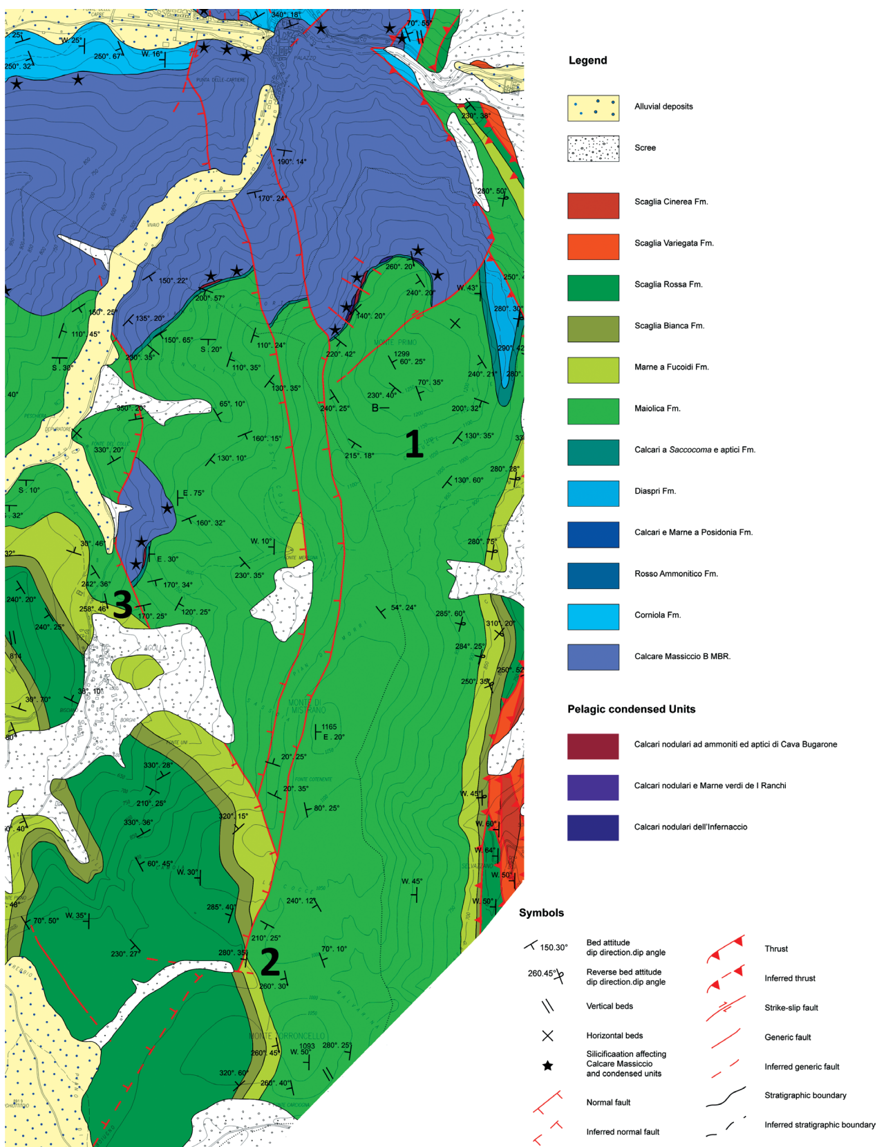
Fig. 2 - Geological map of the study area with the location of the studied stratigraphic sections marked by numbers: 1 - Mt. Primo section; 2 - Mt. Mistrano section; 3 - Agolla section (modified after Fabbi, 2015).
