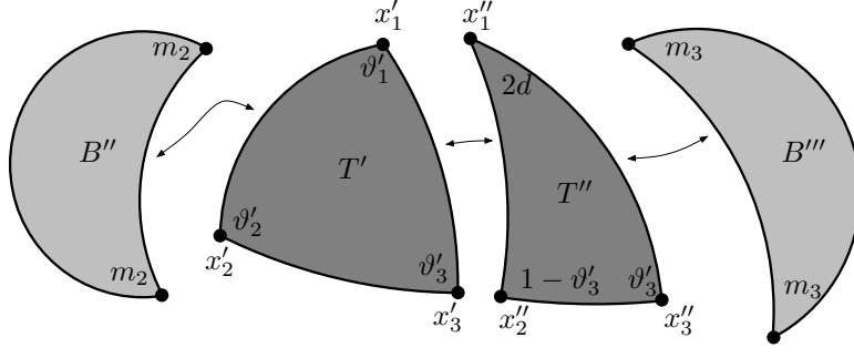
Figure 6: Building the triangle in case (a) of Theorem 3.8.
