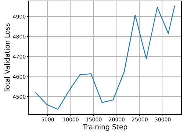
(h) Model DE+\tau+EN^B . Best loss: step 7,200.
