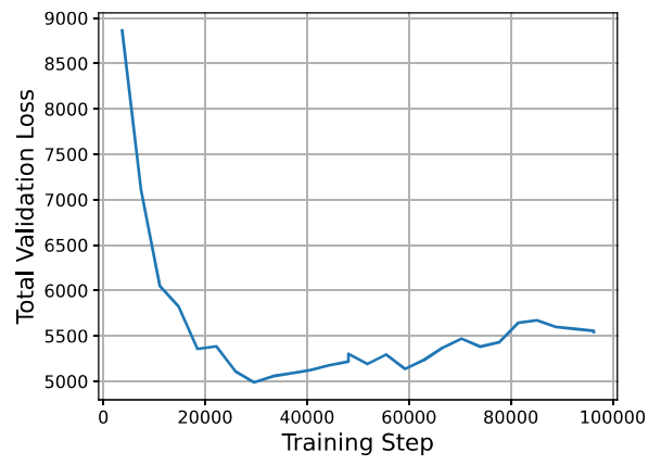
(j) Model DE+\tau+LKEY . Best loss: step 29,600.
