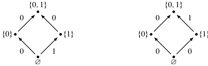
Figure 10: Two (isomorphic) sign assignments on the poset (\emptyset, \{0, 1\}, \subseteq) .
