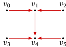
Figure 6: A figure H-type digraph.
