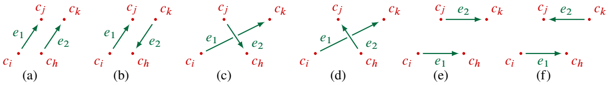
Figure 17: A schematic description of the subcases of case (B) up to a global change in the orientations of e_1 and e_2 .
