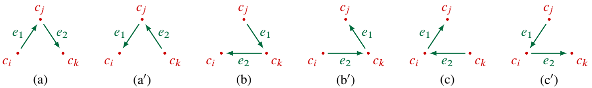
Figure 16: A schematic description of the subcases of case (A). Note that, since the merge of the components c_i, c_j, and c_k must be a path, all possible orientations of e_1 and e_2 are precisely those illustrated.
