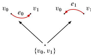
Figure 9: The path poset of the digon graph P_1 in Figure 3.
