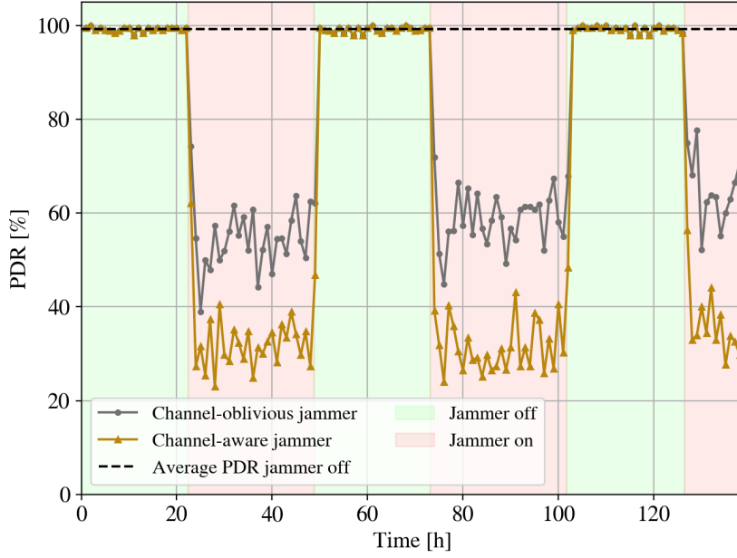
Figure 8.6: Packet Delivery Ratio (PDR) comparing the impact of channel-oblivious jammer, channel-aware jammer and without external interference.
