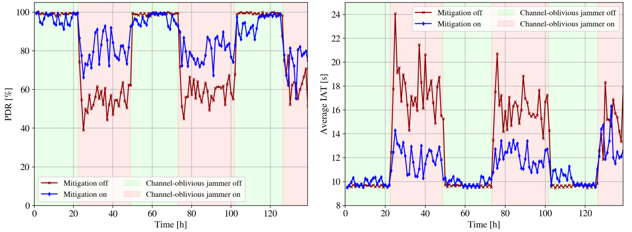
(a) Comparison of Packet Delivery Ratio (PDR) with and without mitigation during channel-oblivious jamming. (b) Average IAT analysis with and without mitigation during channel-oblivious jamming.
