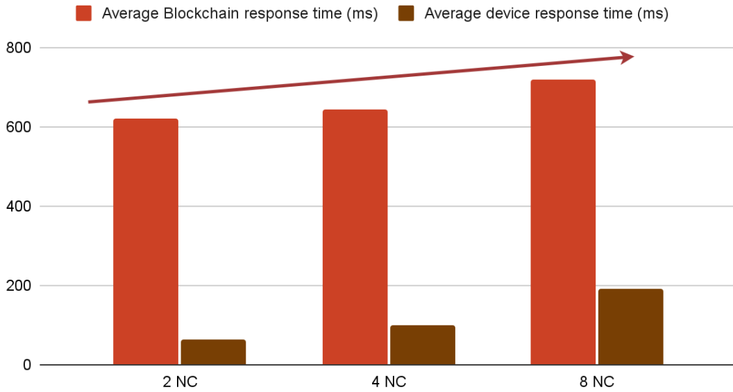
Figure 7.4: DeLoRaN delays with increasing NCs number. It shows the response times of the network controllers as the number of controllers increases exponentially. The response times increased slightly across all configurations, indicating that the system can efficiently distribute the load across multiple controllers without significant performance degradation.
