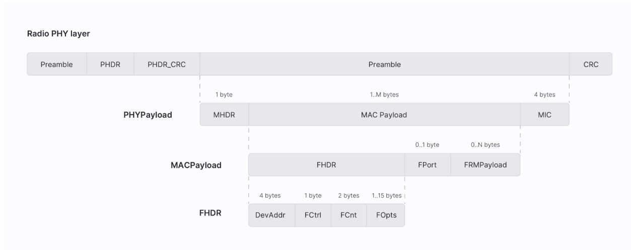
Figure 3.6: The structure of a LoRaWAN frame. Being built on top of LoRa, the physical layer has the structure of a LoRa frame. Its PHYPayload is then divided into MAC Header (MHDR), MAC payload, and a Message Integrity Code (MIC) to check the integrity of the whole packet. The MAC Payload contains application data, which again is divided into Frame Header (FHDR), FPort (used to distinguish different applications), and its payload
