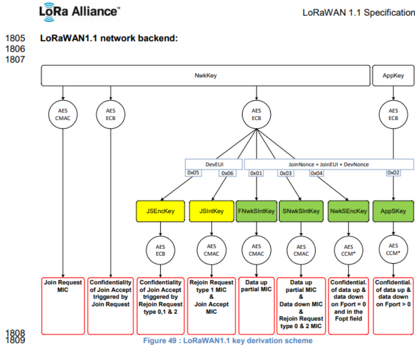
Figure 3.4: The key-derivation scheme used by a LoRaWAN 1.1 ED and NS to calculate the different session keys after a successful join procedure, complete with the goal of each key.
