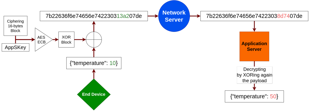
Figure 6.3: Flow of a MITM attack in a centralized LoRaWAN network. The compromised NS has full control of the payload and can alter the data before forwarding it to the AS. The AS is unable to detect the tampering, allowing the attacker to manipulate the communication without detection.
