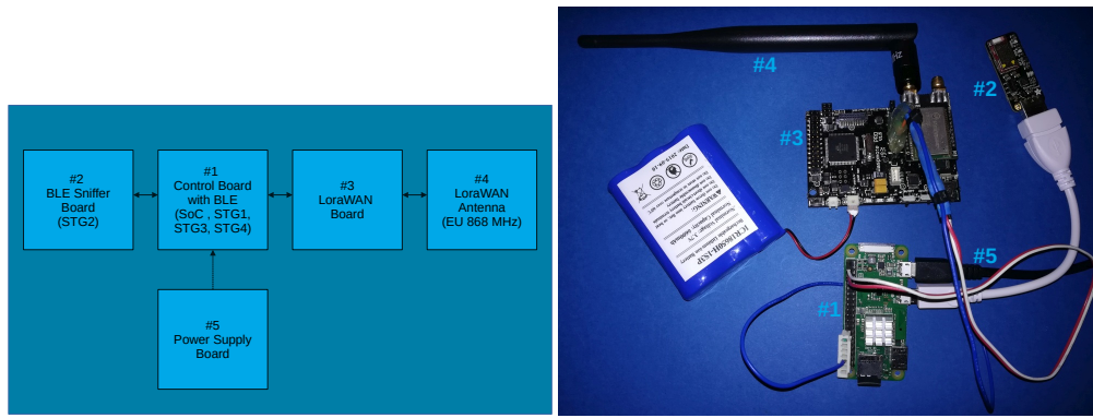
(a) BLENDER station diagram, showing the (b) BLENDER station setup and its components. Even in its PoC state it shows how little a BLENDER station can be.
